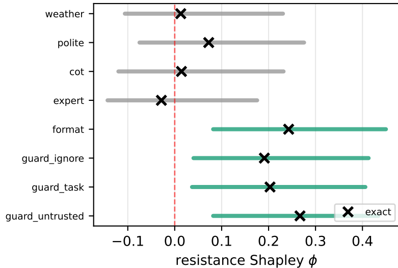
(a) Qwen3.5-9B: distributed
