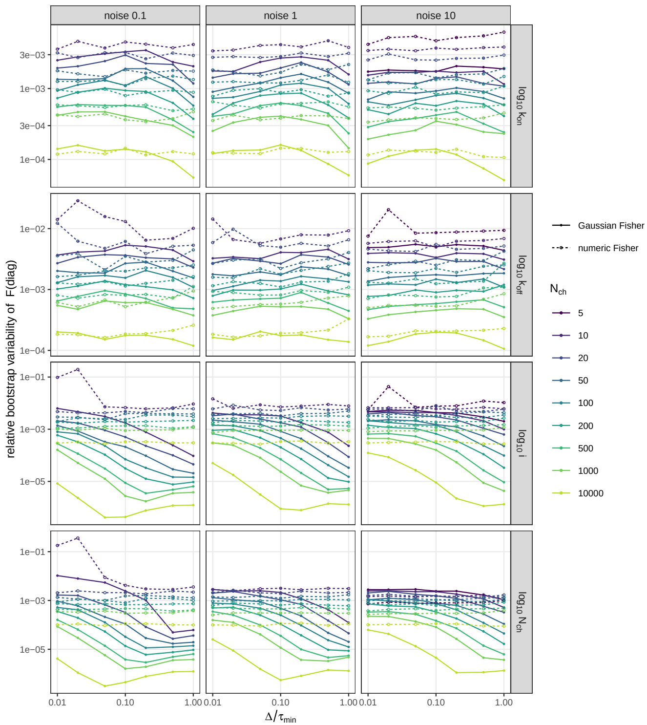
macro_IR Fisher variability: Gaussian (solid) vs numeric (dashed)
