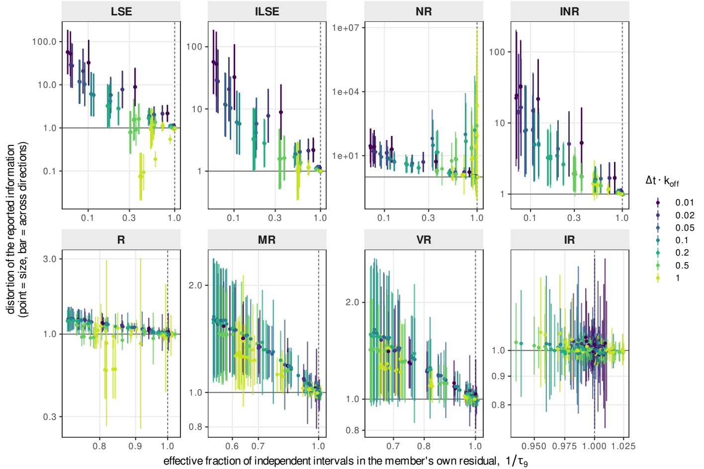
Figure 15. Each member against the memory left in its own residual. The whole ladder, with the horizontal axis of each panel now 1/\tau_0 of that member's own standardized residual, which a reader cannot compute without running the member: a mechanism panel rather than a decision one, and it runs the same way as Figure 13. It asks whether the memory a member fails to remove predicts the information it then misreports. The ladder is ordered by how much each fails to remove: IR occupies a point, its own \tau_0 running 0.98 to 1.07 over the whole plane, R reaches 1.39, and the two least-squares arms span to 17.4. Within a member the prediction holds at a fixed sampling interval, the rank correlation between own memory and own distortion reading +0.92 for ILSE, +0.96 for INR, +0.93 for MR and +0.91 for VR over the whole plane and about +0.99 within one interval. It is necessary and not sufficient: NR carries 73 cells whose own \tau_0 is below 1.05, an eighth of them distorted, and they sit at the two coarsest intervals, where consecutive samples are a relaxation time apart and there was no memory to remove. Each panel is on its own scales.
