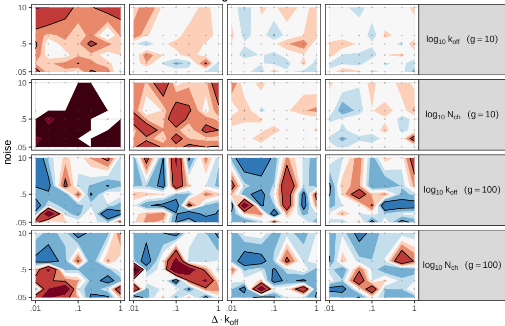
B excess kurtosis of the MLE marginal
