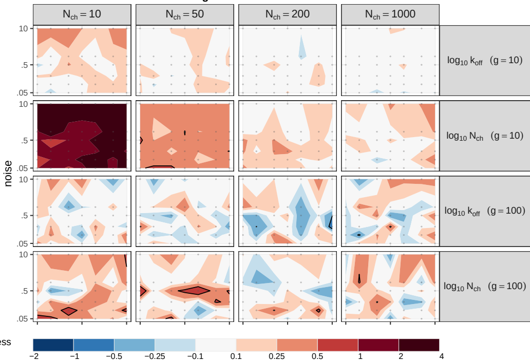
B excess kurtosis of the MLE marginal
