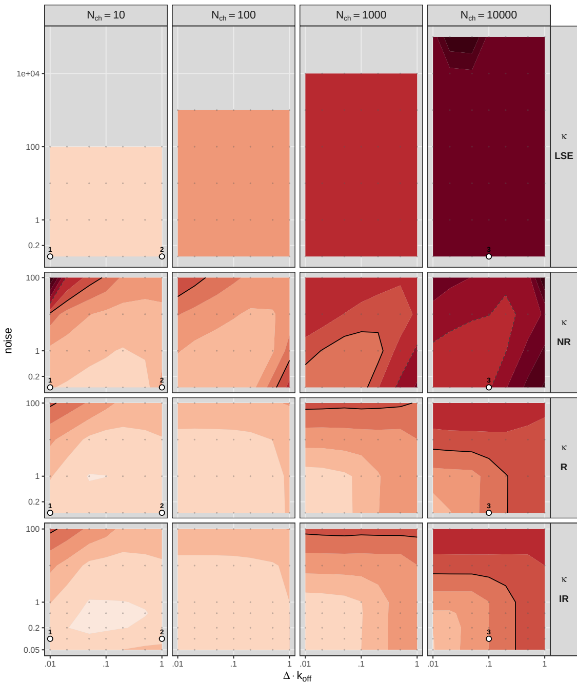
Condition number of the Gaussian Fisher
