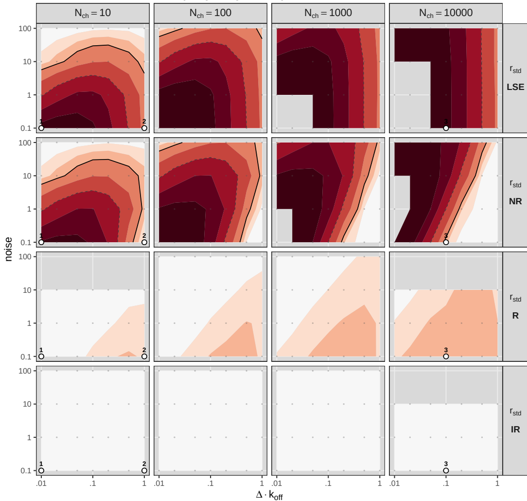
Residual autocorrelation (integral lag of r_{\text{std}} )
