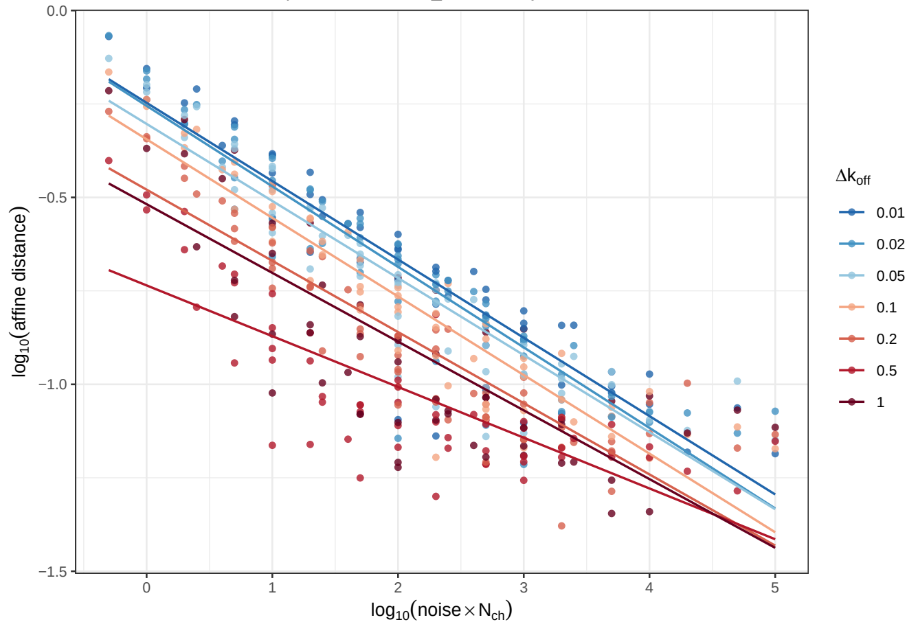
IR residual distortion collapses on noise \times N_{\text{ch}} , offset by interval
