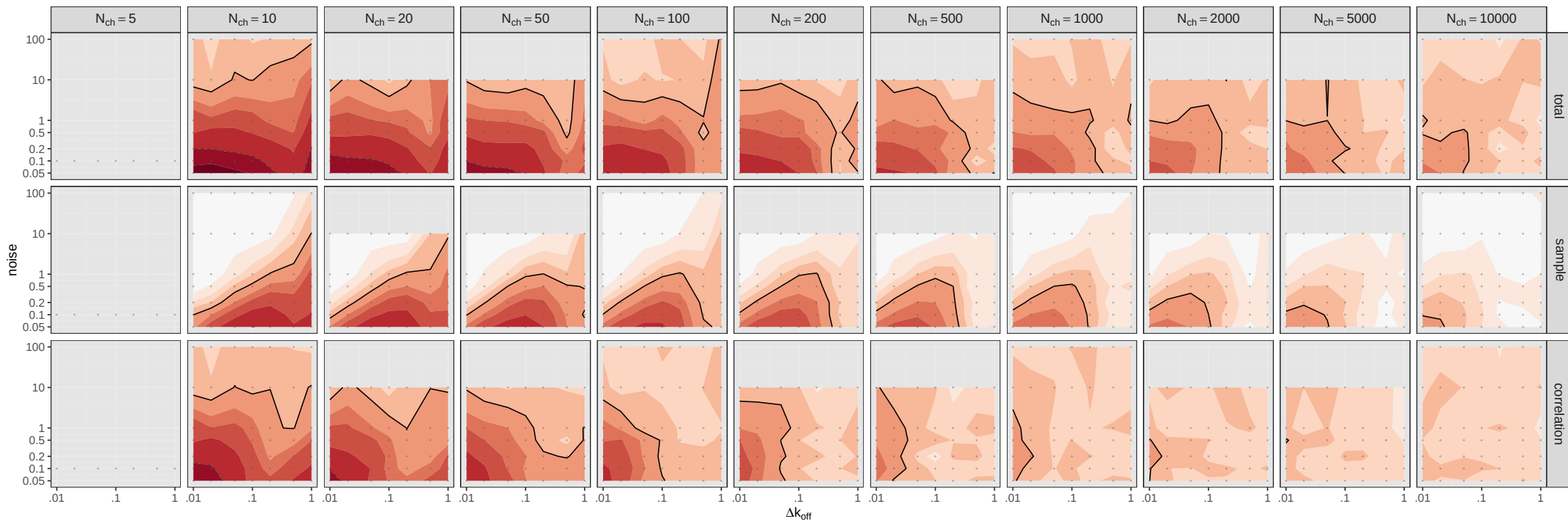
IR validity map: affine distortion (rows: total / sample / correlation), by N_ch
