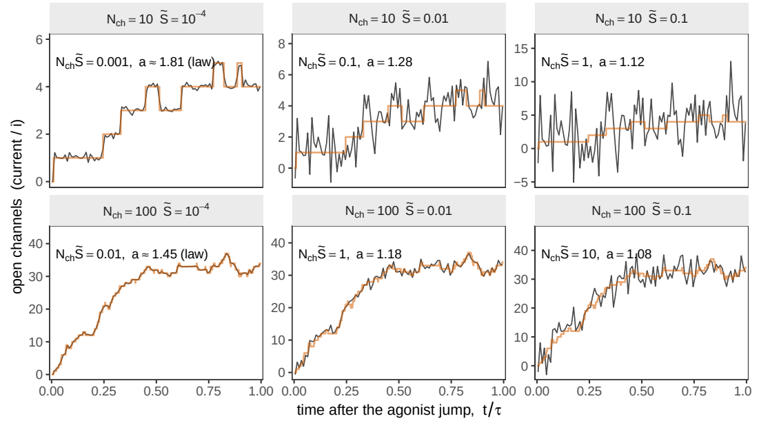
Figure 6—figure supplement 2. What the record looks like on both sides of the limit. Simulated records of the two-state scheme at the sweep's shortest interval, \tilde{\Delta} = 0.01 , for N_{\text{ch}} = 10 and 100 (rows) at \tilde{S} = 10^{-4} , 0.01 and 0.1 (columns), one relaxation time after the agonist jump; grey, the sampled current with the baseline removed, in units of the unitary current; orange, the number of open channels from the simulator's substeps. Each panel gives N_{\text{ch}}\tilde{S} , the noise variance over the life of one conductance level in units of the unitary step, and the anisotropy a measured at that cell and interval. The left column lies a factor of fifty below the sweep's noise floor and carries no measurement: it is what a record that resolves single openings looks like, and its a is the median law of figure supplement 1 extrapolated there (1.81 and 1.45; the 95% line gives 2.11 and 1.60), larger than any value the sweep measured. The sweep's own corner, N_{\text{ch}}\tilde{S} = 0.05 , resolves them only just, with one unitary step per sample of noise, and is where the departure is measured to begin; at N_{\text{ch}} = 100 and \tilde{S} = 0.01 the record follows the count without a visible step and still departs. Same simulator, protocol and seed for every panel (Methods).
