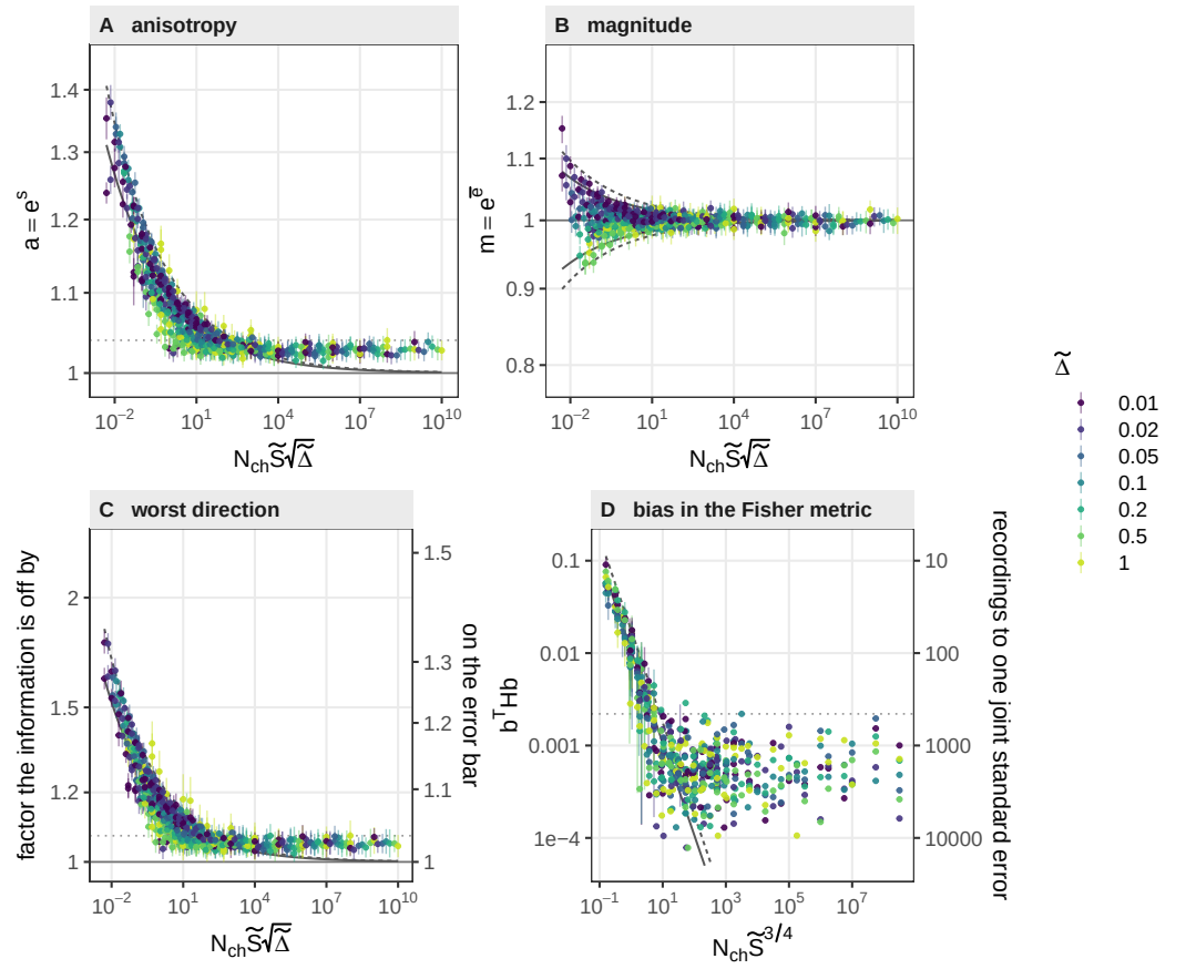
Figure 6—figure supplement 1. The departure of the boundary-conditioned filter: one law, with its spread. All 560 IR cells at the simulation truth, coloured by \tilde{\Delta} . Solid lines are the median law with the slope fixed at -1/5 ( -1 in D), dashed the 95% quantile of the cells about it, dotted the resolution of 10^4 recordings; bars are 95% bootstrap intervals over the recordings. (A) The anisotropy a and (B) the magnitude m of Eq. 4 against x = N_{\text{ch}} \tilde{S} \sqrt{\tilde{\Delta}} , the lines of |\log m| drawn on both sides of one. (C) The worst single direction, the factor by which its information is misreported (right axis, on the error bar). (D) The bias in the Fisher metric per recording, b^T \mathbf{H} b (Appendix 3), against N_{\text{ch}} \tilde{S}^{3/4} ; right axis, its reciprocal, the recordings a pooled fit holds before its bias reaches one joint standard error. All four are read over every direction; Figure 7's calibration line is a per-parameter crossing at the pooled optimum, with its own slope.
