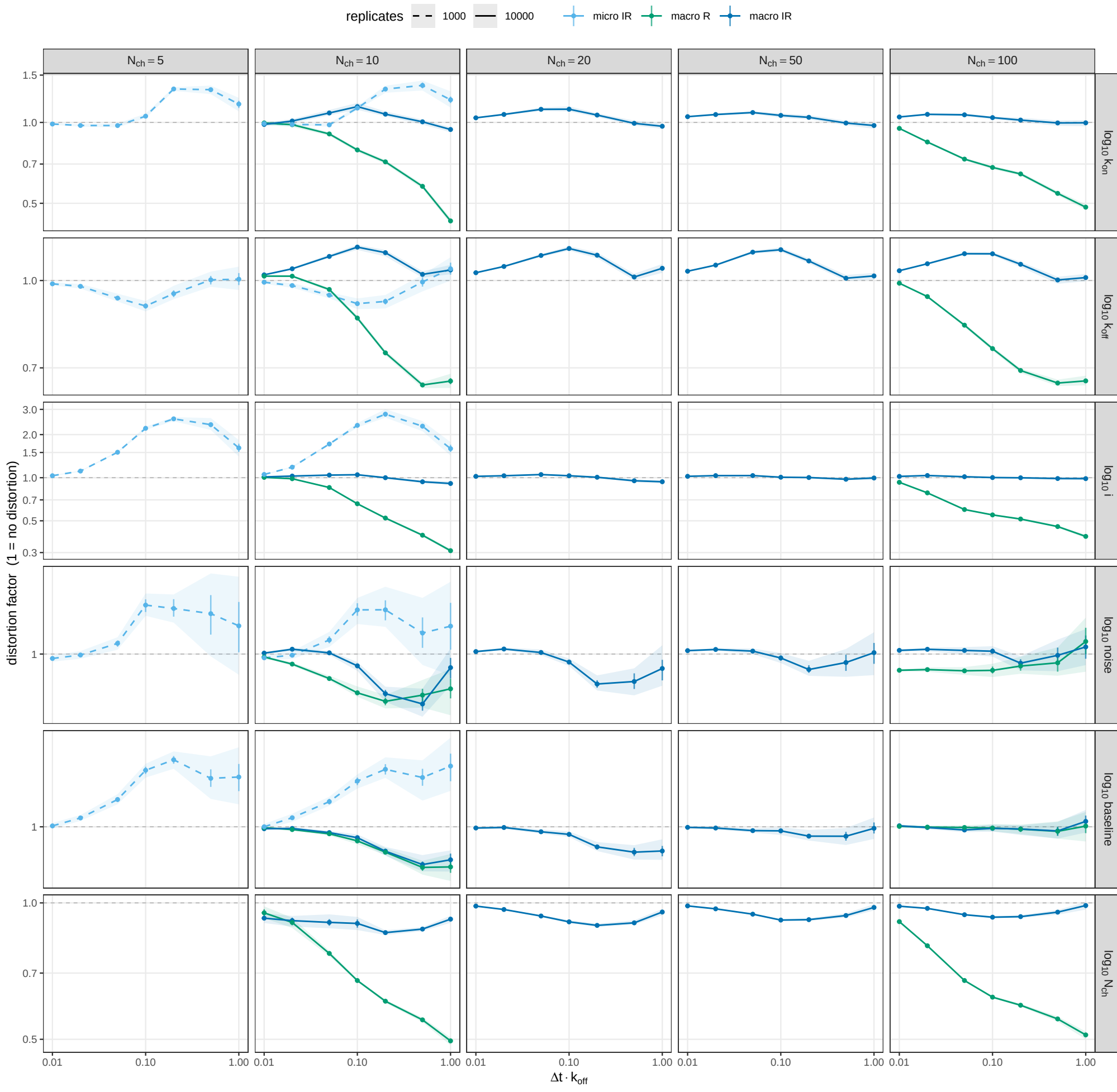
Gaussian sample distortion (diagonal)
