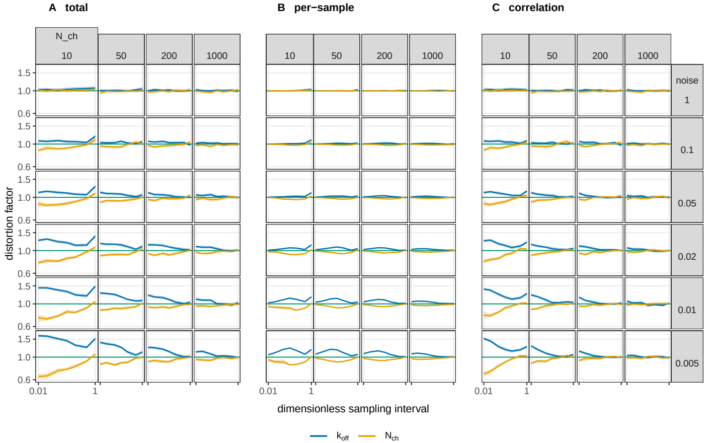
Figure 17. Where the boundary-conditioned filter stops reporting a calibrated error bar, and which of the two discarded moments is responsible. The same measurement as Figure 8, the Gaussian information distortion at the pooled optimum on the same runs, resolved on the corner where IR departs: on Figure 8's scale a factor of 1.5 is a faint tint and here it needs an axis. The three blocks are the distortion and the two parts it decomposes into: (A) the total, (B) the part carried by the per-sample non-Gaussianity of the score, and (C) the part carried by its correlation across intervals; their product reproduces the total to within 1% over the whole grid. Each block is a grid of the design plane in the orientation of Figure 19: the channel count increases to the right, the dimensionless noise \tilde{\sigma} increases upward, and inside every cell the horizontal axis is \tilde{\Delta} from 0.01 to 1, shared by every panel and labelled once per block. The vertical axis is the distortion factor on a logarithmic scale, shared by all twelve columns so that they can be compared, with the green line at 1 marking a report that is neither over- nor under-confident. Colour is the parameter. Bands are 95% percentile bootstrap intervals over recordings, of median half-width 0.03. The two readings the figure supports, and the limits on them, are in the text.
