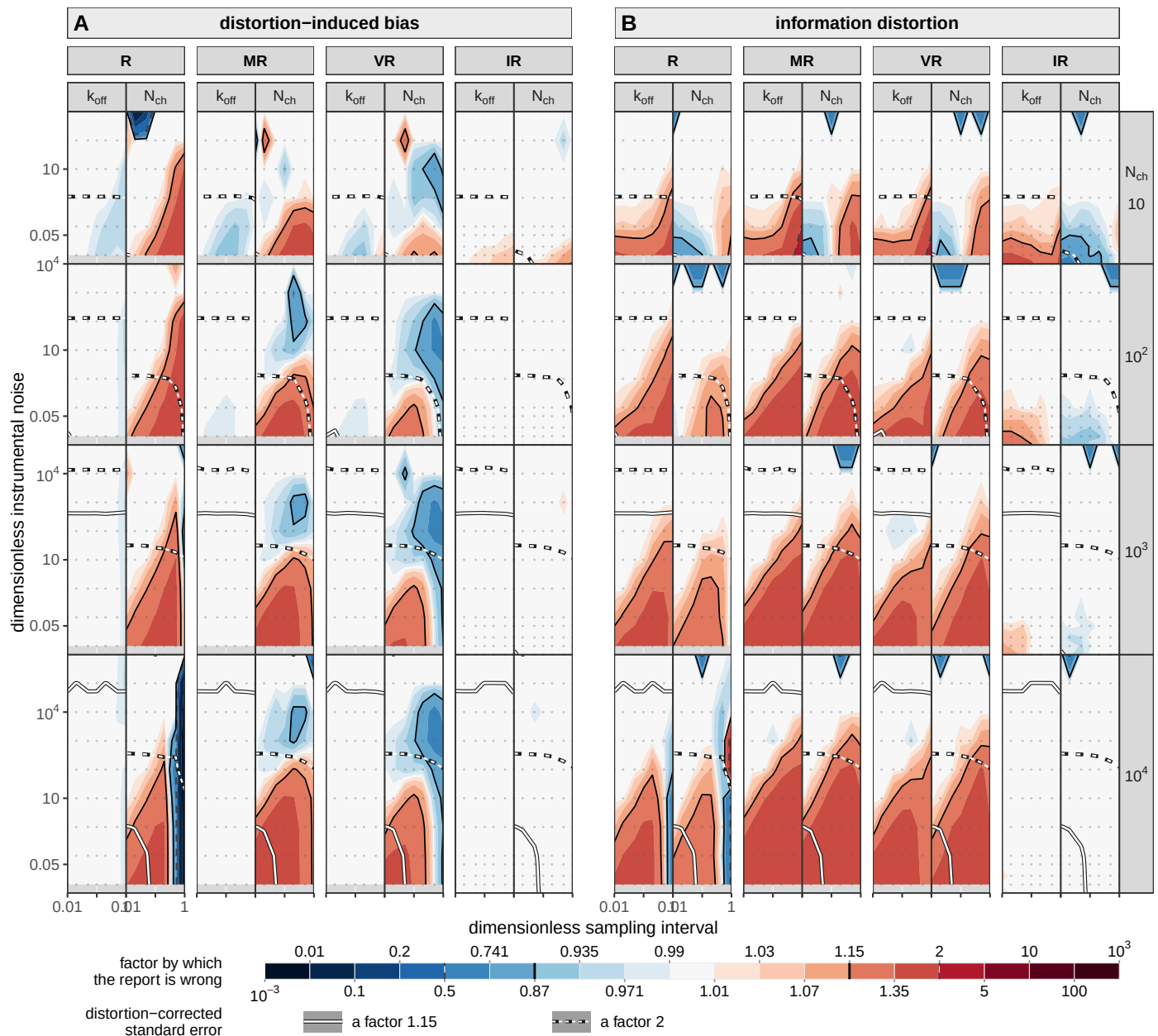
Figure 10. The same plane for the recursive family: R, MR, VR and IR. Figure 8 unchanged in every respect but the roster, the same two moments on the same shared factor scale with the same two line families and the same nesting, over the four rungs inside the recursive family, R, MR, VR and IR (Table 1). Sixteen columns rather than Figure 8's twenty, since no least-squares arm appears and every member carries the channel number. The reading is in the text: each partial correction buys part of the first moment and gives it back in the second as channels are added, and neither approaches either interval member on either moment.
