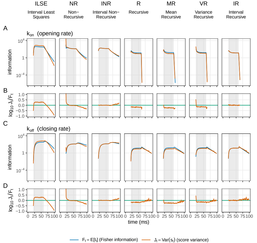
Figure 5. Per-step information against score variance, the opening rate and the closing rate. Seven members across the columns, the least-squares arm being the interval-averaged ILSE, and two parameters down the page as bands of two rows: k_{on} (A, B) and k_{off} (C, D). The upper row of each band carries the per-interval Fisher information and the score variance as magnitudes, which lie on each other where the member is calibrated at that interval; the lower row is \log_{10}(J_i/F_i) with its 95% bootstrap interval, zero when they do. Per-interval calibration is not monotone along the cost ladder: on k_{off} the median reads +0.184 for ILSE, -0.038 for NR, +0.007 for INR, -0.145 for R, -0.229 for MR, -0.135 for VR and +0.033 for IR. Curves stop at the information mask, which is also where the upper axis ends. The least-squares ratio row is the same curve in every band of both halves, median 0.184: with a single constant variance the parameter cancels out of the ratio, leaving the true residual variance over the assumed one.
