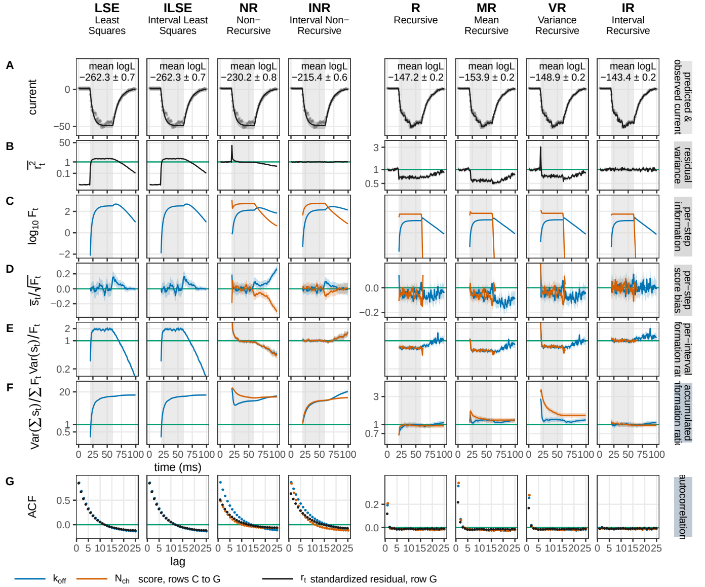
Figure 4. The calibration cascade in time. One set of 1,000 recordings ( N_{\text{ch}} = 100 , \tilde{S} = 0.01 , \tilde{\Delta} = 0.1 ) is scored by each of the eight members, in cost-ladder order and with no fitting. Rows A and B are properties of the data, in grey; C to G are per parameter, the closing rate and the channel number in colour. (A) An example recording, its band the member's own predictive \pm 1 s.d., annotated with the ensemble-mean log-likelihood. (B) The mean squared standardized residual. (C) The per-interval Fisher information. (D) The mean per-interval score over \sqrt{F_t} , standardized so that the two parameters share an axis. (E) The per-interval information ratio \text{Var}(s_t)/F_t . (F) The same ratio accumulated, J_T/F_T . (G) The autocorrelation against lag, of the residual in black and of the score in colour. Bands are 95% bootstrap intervals over the recordings and curves stop where the information reaches the numerical floor, which is also where an interval stops counting as informative in the text and in the source data. Non-negative quantities are on a logarithmic axis and signed ones on a linear axis, with the calibrated value on the ticks; the four open-loop columns share a y-scale block distinct from the four recursive ones.
