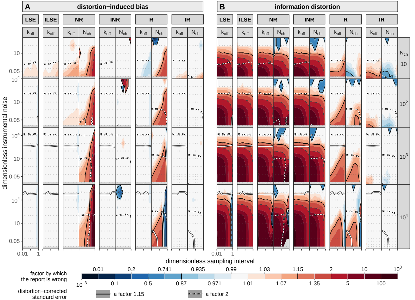
Figure 8. The design plane: how wrong each member's report is, in both moments, on one scale. Ten thousand recordings are simulated at every cell of the grid and scored by each member of the cost ladder. (A) The distortion-induced bias, evaluated at the simulation truth \theta_{\text{sim}} : how far the estimate is displaced. (B) The information distortion, evaluated at the pooled optimum \theta_{\text{pool}} (Methods): how far the uncertainty a member reports is from the one it delivers. Columns nest twice, member and then parameter, k_{\text{off}} and N_{\text{ch}} . Both least-squares arms are on the grid and each holds one column per half rather than two, their four-parameter configuration fixing the unitary current and the noise level at the simulated values (Methods). Rows are the channel count, each given a height proportional to the range of instrumental noise the sweep reaches there. Inside a panel the axes are the sampling interval in units of \tau and the dimensionless instrumental noise, one decade the same distance on both. Colour is shared by the two halves: the factor by which the report is wrong, centred on one, pale right and saturated wrong in either direction, blue conservative, clipped at 10^{\pm 3} . What a factor means differs between them: in (A) it is a factor on the parameter, so 2 means the estimate is out by a factor of two, while in (B) it is a ratio of variances, so 2 means the reported error bar is \sqrt{2} , about 40%, too narrow. Lines carry two codes: colour says which quantity, dark hairlines cutting the colour field and white lines on a dark casing cutting the distortion-corrected standard error, which asks whether the parameter can be measured at all rather than whether its error bar is calibrated; dash says which criterion, solid a factor 1.15 and dashed a factor 2, the two thresholds used throughout.
