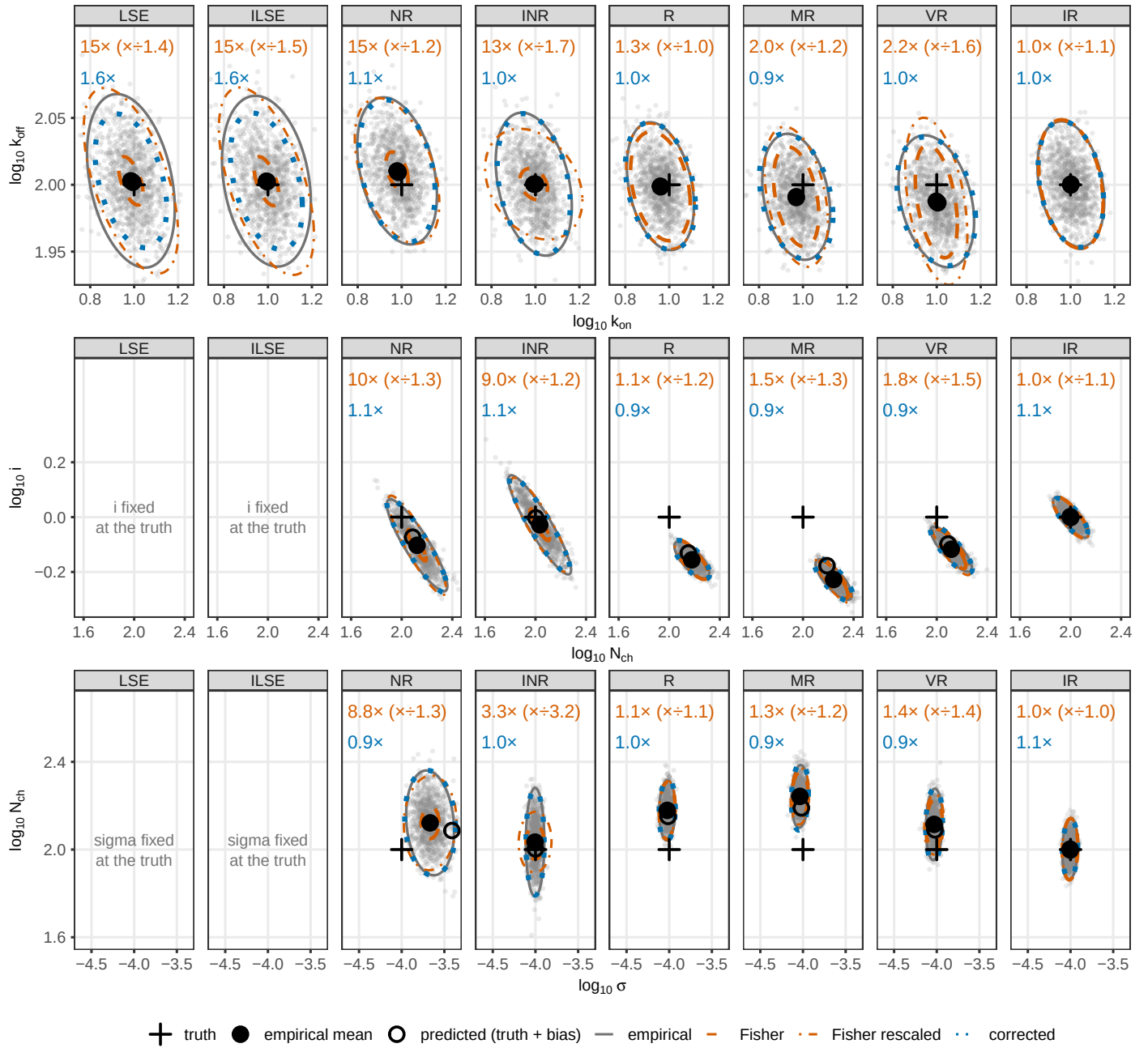
Figure 2. Parameter recovery and the calibration of the reported interval, for the whole ladder at one design cell. N_{\text{ch}} = 100 , \tilde{S} = 0.01 , \tilde{\Delta} = 0.1 ; 10,000 recordings in groups of ten, so one thousand maximum-likelihood estimates per member. Columns are the eight members in ladder order, rows the kinetic, amplitude and noise pairs, with \sigma the instrumental noise level. Each panel carries the cloud of estimates and four 95% ellipses at its mean, named in the key. Above the cloud, the orange numbers are the magnitude of the distortion and, in parentheses, its anisotropy; the blue number is the empirical ellipse over the corrected one. All three read 1.0 for a calibrated member. Covariances are the Gaussian-Fisher family at the pooled estimate, divided by the group size.
