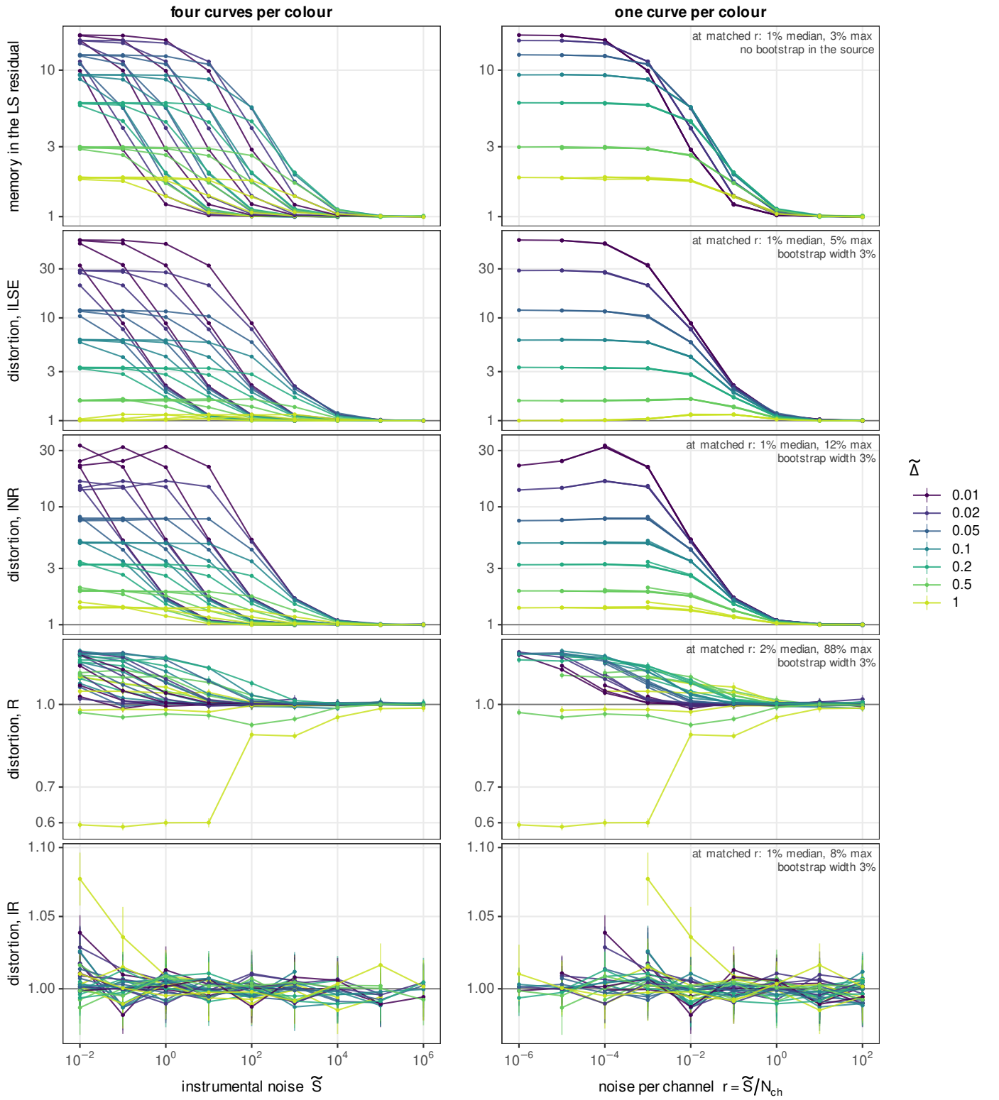
Figure 14. The instrumental noise and the channel count act only through their ratio. The same cells as Figure 13, drawn twice. Each line is one channel count at one acquisition interval swept over the instrumental noise, twenty-eight per panel, and the two columns differ in nothing but the horizontal coordinate: on the left the instrumental noise \tilde{S} , on the right the noise per channel r = \tilde{S}/N_{\text{ch}} . On the left the four channel counts are four separate curves per colour, a decade apart; on the right they merge, so seven of the twenty-eight are visible. Nothing is fitted, rescaled or normalized between the columns. The top row is the quantity Figure 13's horizontal axis inverts, \tau_9 of the least-squares residual, and it collapses with the rest: a reader who measures \tau_9 on their own record has measured r without knowing it. The vertical bars are the bootstrap quantiles of each cell, absent on the top row alone: each point is known to about 3% and the four channel counts land within 1% of one another. The number in each right-hand panel is the residual disagreement between cells that share r exactly at the same interval, with no interpolation. The 5% of ILSE and the 8% of IR are within that scatter; the one large value, R's, is the single ill-conditioned cell at N_{\text{ch}} = 10^4 and \tilde{\Delta} = 1 that Figure 8 paints
