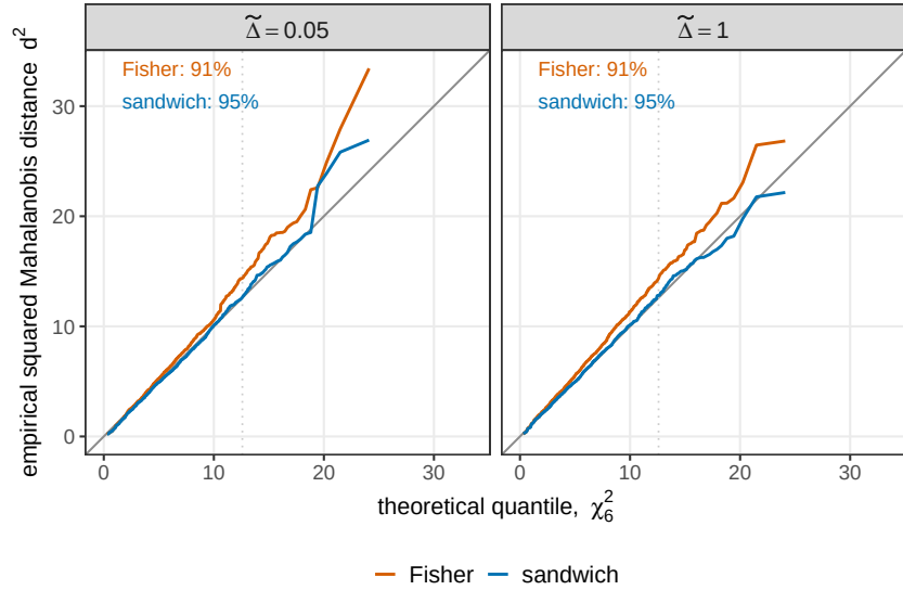
Figure 3. The reported covariance against the empirical one, in all six directions at once. The squared Mahalanobis distance of each estimate from the cloud mean, sorted and drawn against the quantiles of a \chi^2 with six degrees of freedom, under the covariance the member reports and under the distortion-corrected sandwich. A calibrated covariance lies on the identity; above it the reported region is too small and under-covers. The reported Fisher covariance under-covers the nominal 95% region and the sandwich covers it, 0.914 against 0.947 to 0.949. Centring on the cloud mean tests the second moment alone, which is what the correction claims to repair. Each panel is one acquisition interval, \tilde{\Delta} = 0.05 and \tilde{\Delta} = 1 . Two things differ from Figure 2, both forced by the sample: the member is IR alone, and the cell is N_{\text{ch}} = 10 at \tilde{\Delta} = 0.005 with group size 100, the one cloud in the set carrying a thousand fits of that size.
