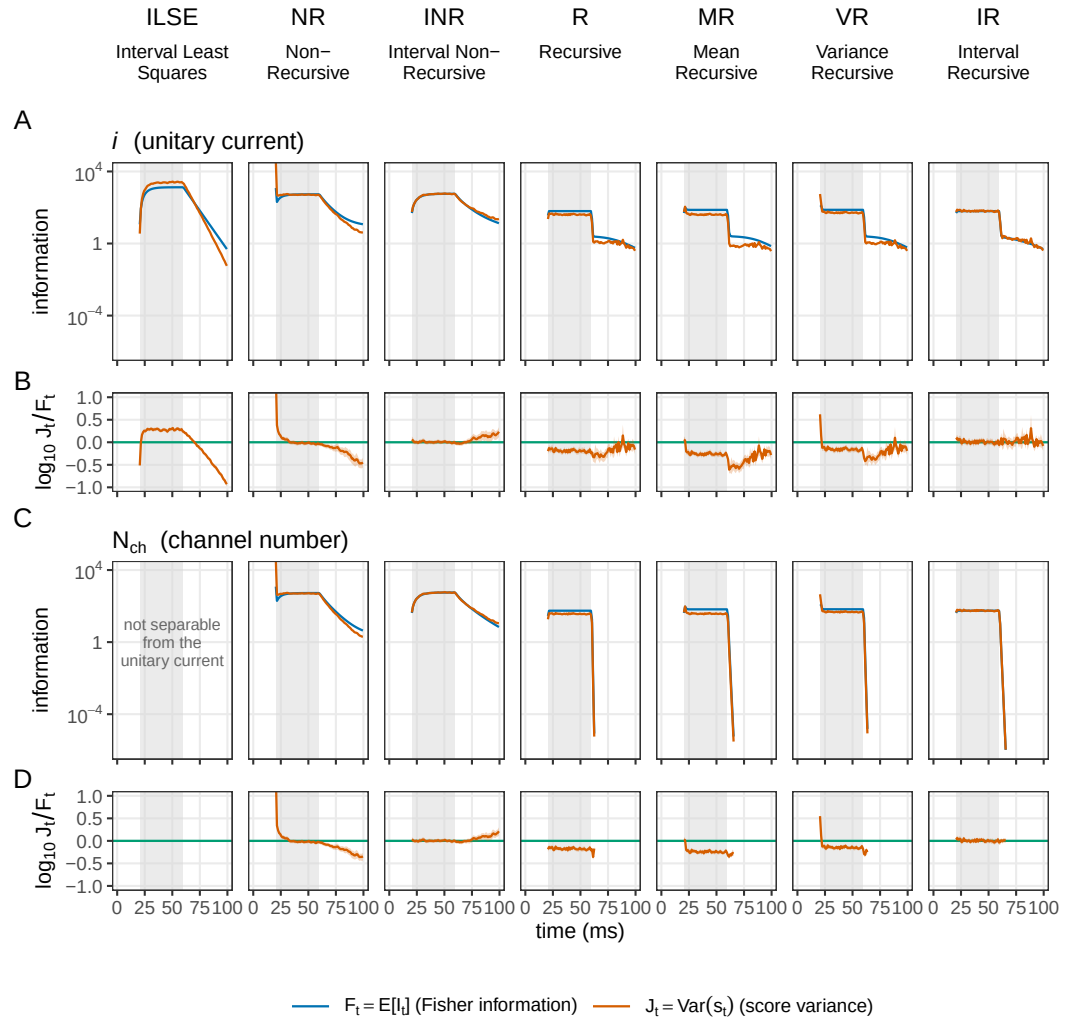
Figure 6. Per-step information against score variance, the unitary current and the channel number. The other half of Figure 5, on the same seven members of the likelihood ladder, read the same way: the unitary current (A, B) and N_{ch} (C, D), the upper row of each band the per-interval Fisher information against the score variance and the lower row \log_{10}(J_t/F_t) with its 95% bootstrap interval. In the two recursive columns the N_{ch} band reaches the information floor within six intervals of washout while the unitary-current band does not. The channel-number band carries no least-squares panel: N_{ch} is not separable from i there.
