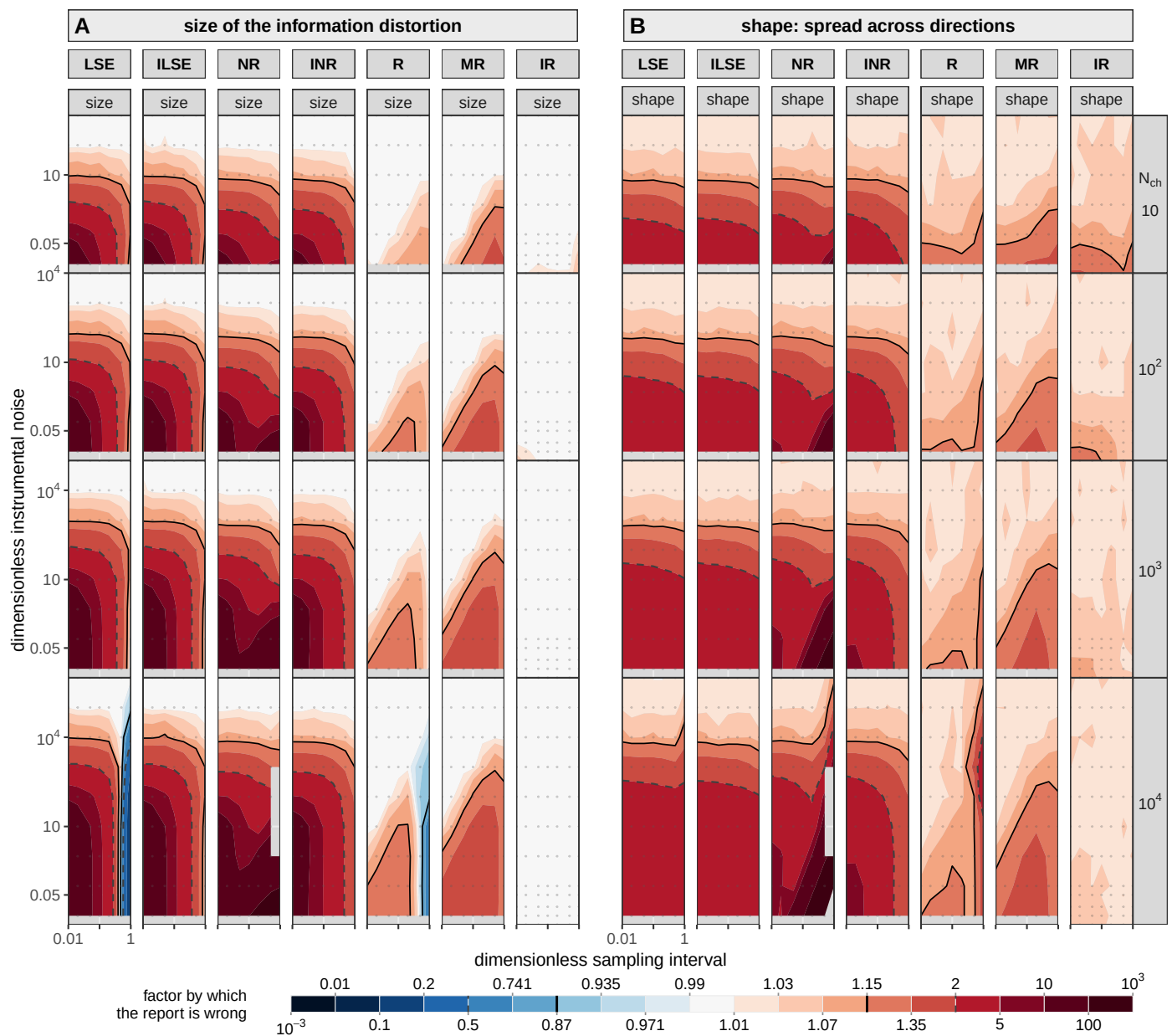
Figure 11. The magnitude of the information distortion against its anisotropy. Two invariants of the same distortion matrix over the same plane, for seven members: both least-squares arms, NR, INR, R, MR and IR. (A) its magnitude m and (B) its anisotropy a (Eq. 4), m signed about a null of one and a one-sided. The rule they give: a at one means a single effective-count rescaling is exact and m is the factor it should use; a above one means no such rescaling exists at any factor. The two least-squares arms are the same figure wherever the recording is finely sampled, and part at the coarsest interval: at \tilde{\Delta} = 1 and 10^4 channels LSE reads 0.074 in magnitude, understating its own information thirteenfold, where ILSE reads 1.00. That is the mean model failing and not the variance model, and it is the deepest of the few cells anywhere on this page where a member is conservative rather than overconfident: 11 of LSE's 210 cells and 4 of R's, all of them at the two coarsest intervals and none for any other member.
