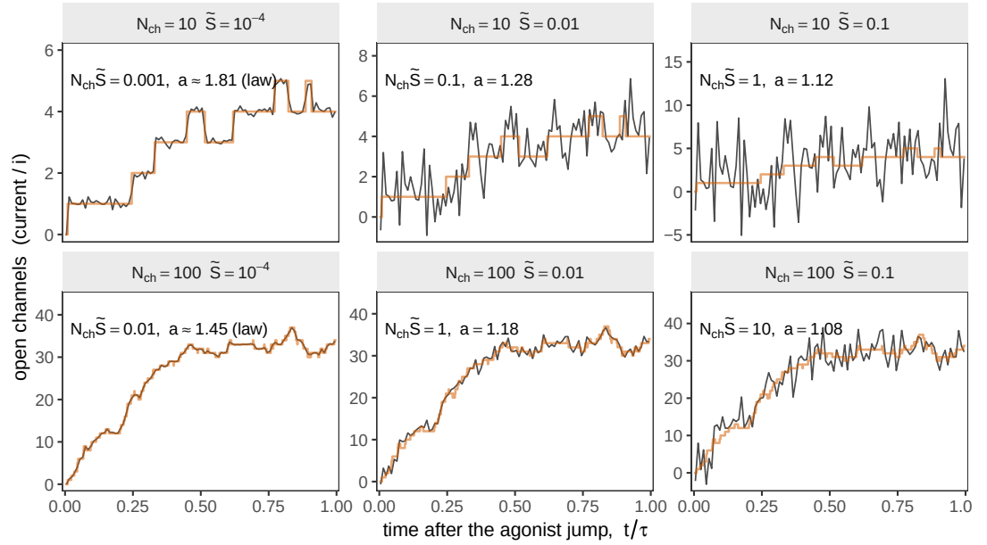
Figure 16. What the record looks like on both sides of the limit. Simulated records of the two-state scheme at the sweep's shortest interval, \tilde{\Delta} = 0.01 , for N_{\text{ch}} = 10 and 100 (rows) at \tilde{S} = 10^{-4} , 0.01 and 0.1 (columns), one relaxation time after the agonist jump; grey, the sampled current with the baseline removed, in units of the unitary current; orange, the number of open channels from the simulator's substeps. Each panel gives N_{\text{ch}}\tilde{S} , the noise variance over the life of one conductance level in units of the unitary step, and the anisotropy a measured at that cell and interval. The left column lies a factor of fifty below the sweep's noise floor and carries no measurement: it is what a record that resolves single openings looks like, and its a is the median law of Figure 18 extrapolated there (1.81 and 1.45; the 95% line gives 2.11 and 1.60), larger than any value the sweep measured. The sweep's own corner, N_{\text{ch}}\tilde{S} = 0.05 , resolves them only just, with one unitary step per sample of noise, and is where the departure is measured to begin; at N_{\text{ch}} = 100 and \tilde{S} = 0.01 the record follows the count without a visible step and still departs. Same simulator, protocol and seed for every panel (Methods).
