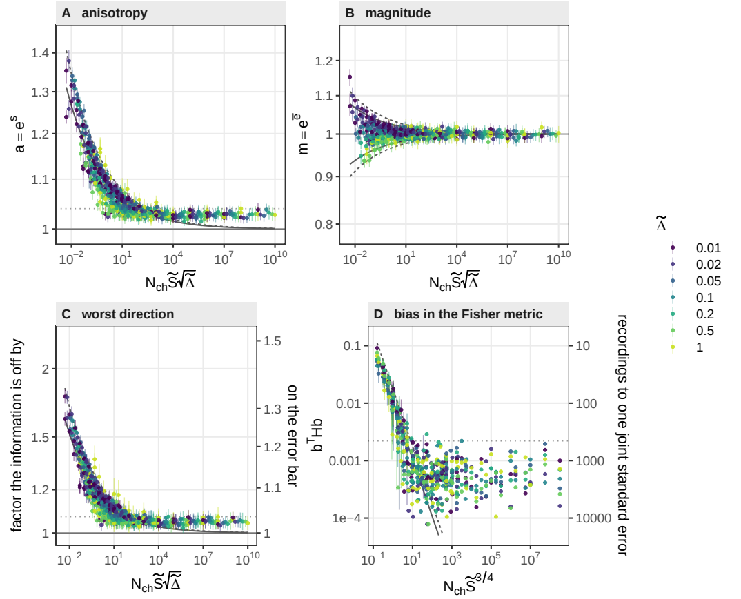
Figure 18. The departure of the boundary-conditioned filter: one law, with its spread. All 560 IR cells at the simulation truth, coloured by \tilde{\Delta} . Solid lines are the median law with the slope fixed at -1/5 ( -1 in D), dashed the 95% quantile of the cells about it, dotted the resolution of 10^4 recordings; bars are 95% bootstrap intervals over the recordings. (A) The anisotropy a and (B) the magnitude m of Eq. 4 against x = N_{ch} \tilde{S} \sqrt{\tilde{\Delta}} , the lines of |\log m| drawn on both sides of one. (C) The worst single direction, the factor by which its information is misreported (right axis, on the error bar). (D) The bias in the Fisher metric per recording, b^T \mathbf{H} b (Appendix 3), against N_{ch} \tilde{S}^{3/4} ; right axis, its reciprocal, the recordings a pooled fit holds before its bias reaches one joint standard error. All four are read over every direction; Figure 19's calibration line is a per-parameter crossing at the pooled optimum, with its own slope.
