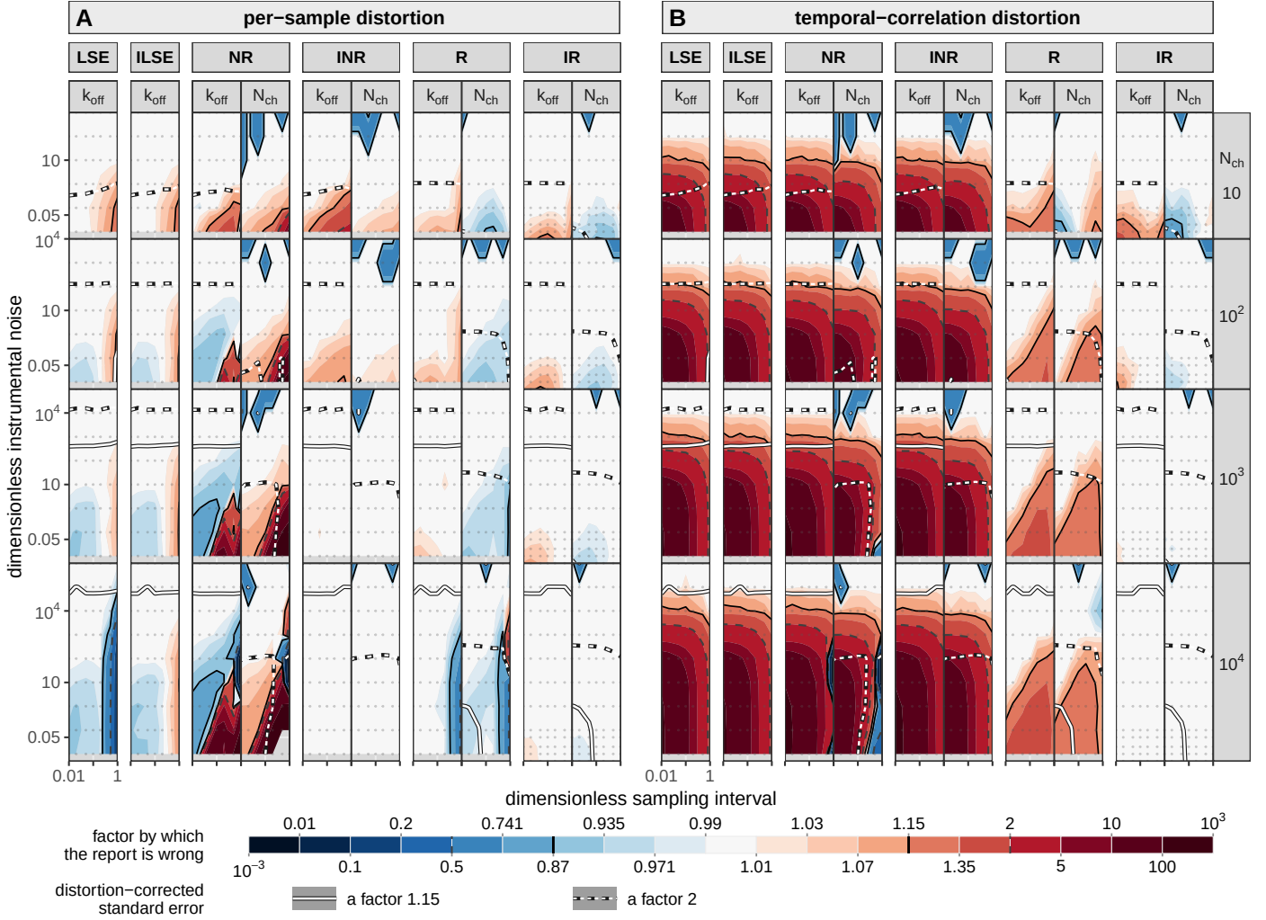
Figure 9. The distortion factored: what is a one-interval failure and what is a failure across intervals.
