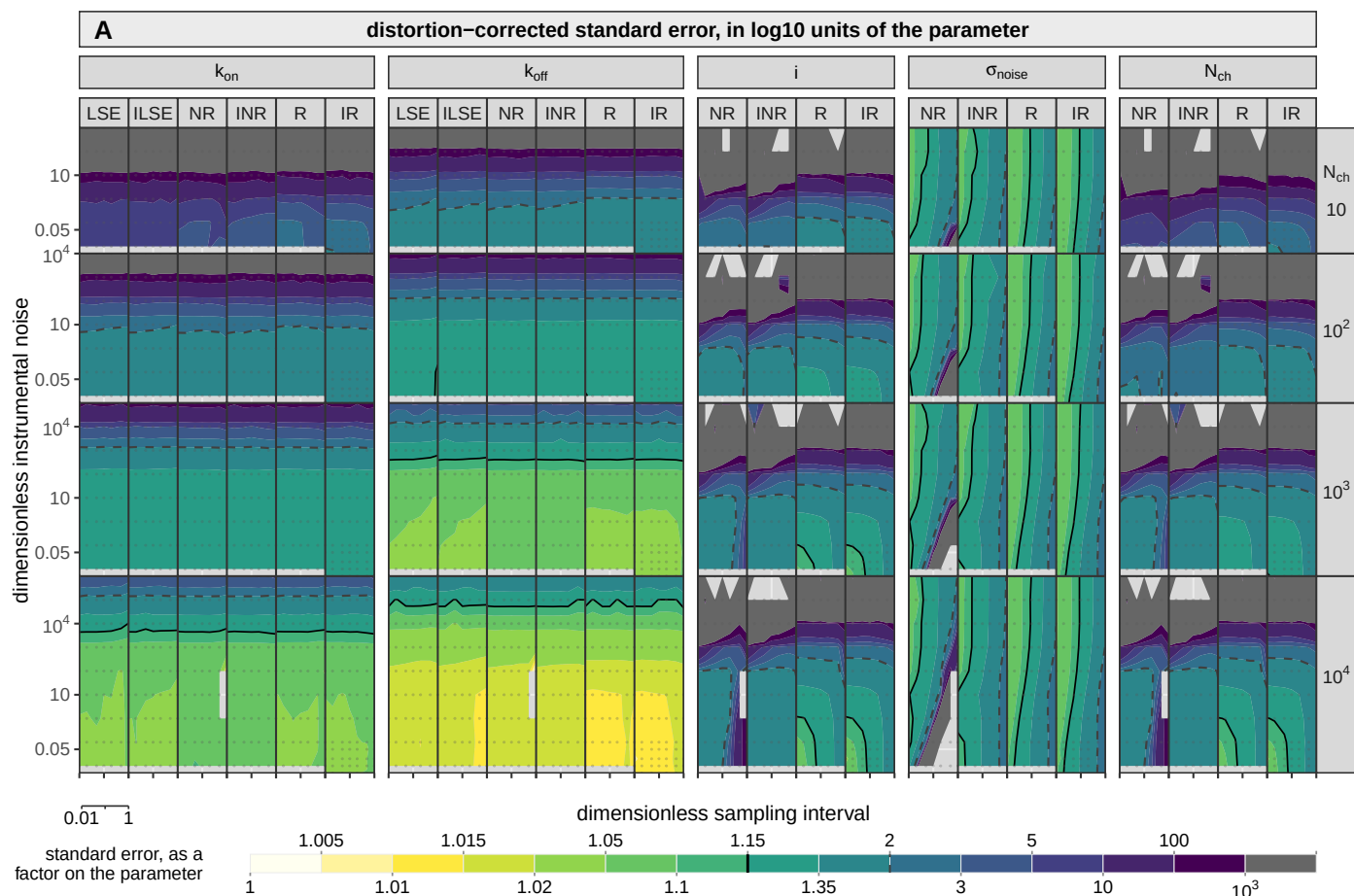
Figure 12. What each member of the likelihood family achieves, as opposed to what it reports. The standard error each member delivers on each parameter: the square root of the diagonal of the distortion-corrected covariance, over the same plane as Figure 8 and in the same orientation. What the design axes buy is read directly off it, and the reading is in the text. It is also the field whose level set at a factor of two draws two of the boundaries of Figure 19. Blocks are per parameter, the members side by side inside each. The scale is sequential: pale is a parameter pinned, dark one barely determined. The two marks are an error bar of 15% of the parameter and an error bar of a factor two. The corrected error is drawn rather than the reported one, which Figure 8 shows wrong by up to a factor of 74, so only the corrected version compares members on the same footing. Both least-squares arms hold the unitary current and the noise level fixed and so appear on the rate blocks alone.
