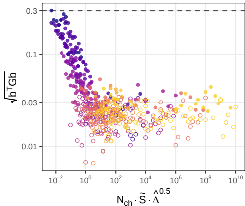
C bias in the Fisher metric
