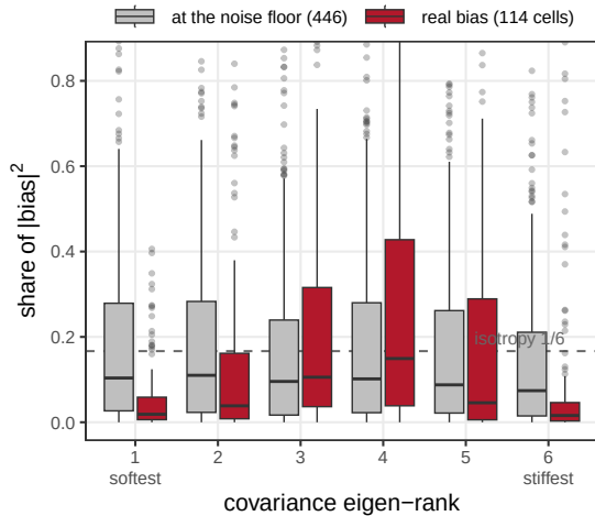
B bias direction: avoids soft and stiff
