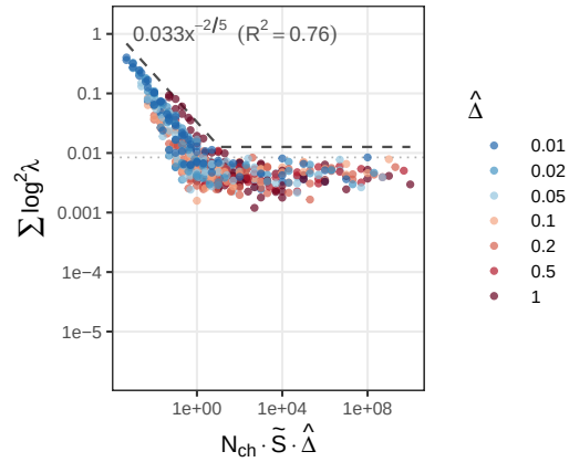
D correlation: \sum \log^2 \lambda
