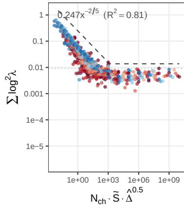
B total: \sum \log^2 \lambda
