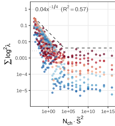
C sample: \sum \log^2 \lambda
