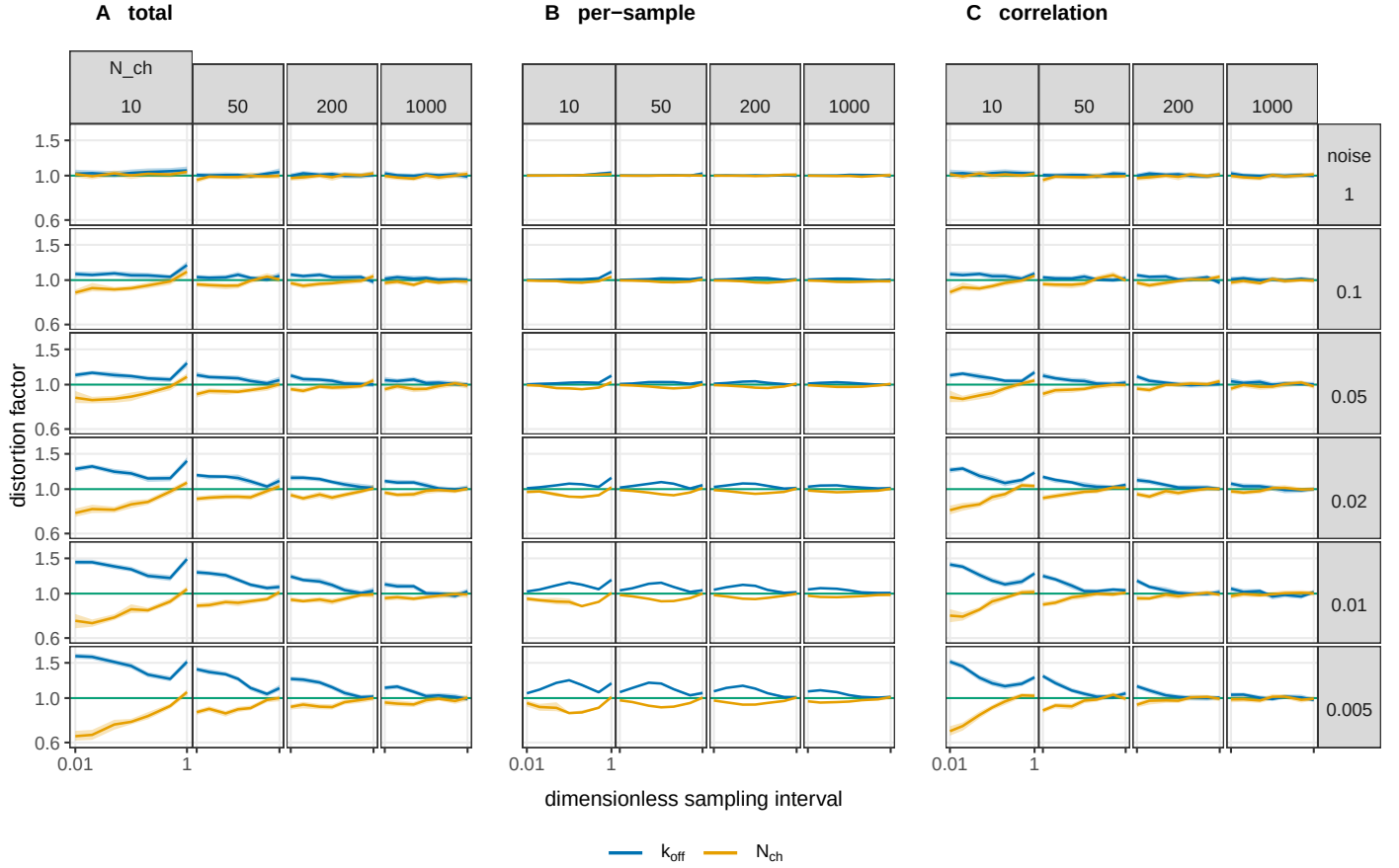
Figure 6. Where the boundary-conditioned filter stops reporting a calibrated error bar, and which of the two discarded moments is responsible. The same measurement as Figure ??, the Gaussian information distortion at the pooled optimum on the same runs, resolved on the corner where IR departs: on Figure ??'s scale a factor of 1.5 is a faint tint and here it needs an axis. The three blocks are the distortion and the two parts it decomposes into: (A) the total, (B) the part carried by the per-sample non-Gaussianity of the score, and (C) the part carried by its correlation across intervals; their product reproduces the total to within 1% over the whole grid. Each block is a grid of the design plane in the orientation of Figures ?? and ??: the channel count increases to the right, the dimensionless noise \tilde{S} increases upward, and inside every cell the horizontal axis is \tilde{\Delta} from 0.01 to 1, shared by every panel and labelled once per block. The vertical axis is the distortion factor on a logarithmic scale, shared by all twelve columns so that they can be compared, with the green line at 1 marking a report that is neither over- nor under-confident. Colour is the parameter. Bands are 95% percentile bootstrap intervals over recordings, of median half-width 0.03. The two readings the figure supports, and the limits on them, are in the text.
