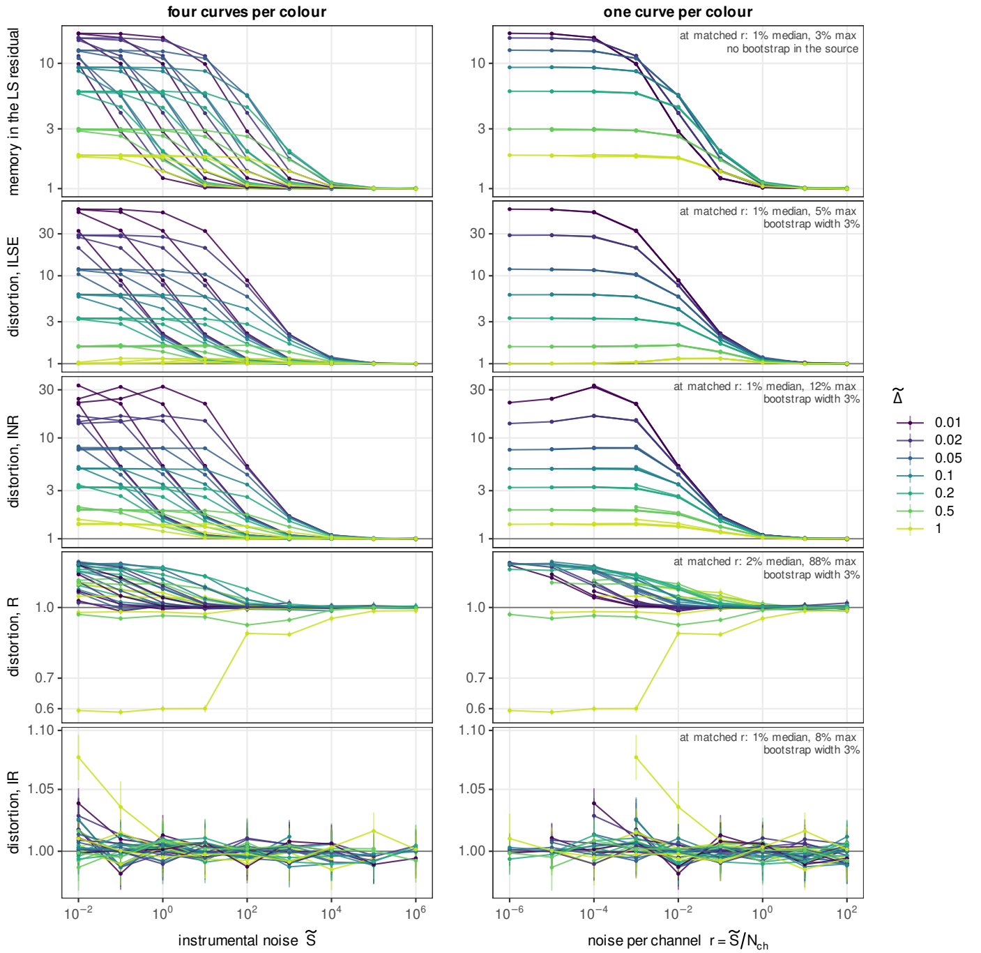
Figure 14. The instrumental noise and the channel count act only through their ratio. The same cells as Figure 13, drawn twice. Each line is one channel count at one acquisition interval swept over the instrumental noise, twenty-eight per panel, and the two columns differ in nothing but the horizontal coordinate: on the left the instrumental noise \tilde{S} , on the right the noise per channel r = \tilde{S}/N_{\text{ch}} . On the left the four channel counts are four separate curves per colour, a decade apart; on the right they merge, so seven of the twenty-eight are visible. Nothing is fitted, rescaled or normalized between the columns. The top row is the quantity Figure 13's horizontal axis inverts, \tau_9 of the least-squares residual, and it collapses with the rest: a reader who measures \tau_9 on their own record has measured r without knowing it. The vertical bars are the bootstrap quantiles of each cell, absent on the top row alone: each point is known to about 3% and the four channel counts land within 1% of one another. The number in each right-hand panel is the residual disagreement between cells that share r exactly at the same interval, with no interpolation. The 5% of ILSE and the 8% of IR are within that scatter; the one large value, R's, is the single ill-conditioned cell at N_{\text{ch}} = 10^4 and \tilde{S} = 1 that Figure 8 paints at the deep end of its scale, without which R agrees to 23%. In the bottom row IR's departures from unity are the width of its own error bar and not structure.
