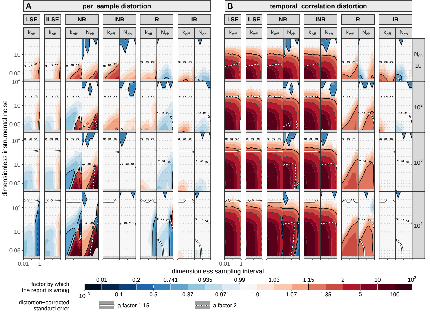
Figure 9. The distortion factored: what is a one-interval failure and what is a failure across intervals. Figure 8's second moment split into the two congruences the battery computes separately, the per-sample part \mathbf{H}^{-1/2} \mathbf{J}_s \mathbf{H}^{-1/2} , the departure of a single interval from the Gaussian the member assumes, and the correlation part \mathbf{J}_s^{-1/2} \mathbf{J} \mathbf{J}_s^{-1/2} , the memory across intervals that a likelihood diagonal in time cannot see (defined above). Same plane, same rows, same scale, same six members and the same two criteria as Figure 8, nested component over member over parameter. Both factors are read at \theta_{pool} , as in Figure 8B. It is the same split Figure 4 measures per parameter from the score, as rows (E) and (F), and read at the truth there rather than at the optimum; the two readings agree for the members that are centred and part company for the displaced ones, so a factor of this figure is not to be matched against a factor of that figure without the anchor. NR and INR carry the same correlation part, 16.5, 19.5, 21.2, 21.2 against 16.5, 20.7, 21.8, 22.1 on the closing rate across the four decades of channel count, as they must, since they differ by a one-interval variance term and by nothing about time; what separates them is the per-sample part, where NR runs 1.24, 1.02, 5.68, 47.2 and diverges while INR runs 1.72, 1.15, 1.02, 1.00 and converges, and on the channel number the same pair ends at 569 against 1.00. The divergence Figure 8 shows for NR is therefore not a temporal failure at all: it is the one-interval variance missing a term that grows with the channel count. The recursion buys the other factor and only the other factor: INR to IR takes the correlation part from 22.1 to 1.000 and leaves the per-sample part where it was. The factorisation is exact in the log-determinant and not entry by entry, the reconstruction being \mathbf{K} \mathbf{K}^T with \mathbf{K} = \mathbf{H}^{-1/2} \mathbf{J}_s^{1/2} : 1.024 \times 1.433 = 1.468 against a total of 1.481 for R at a thousand channels.
