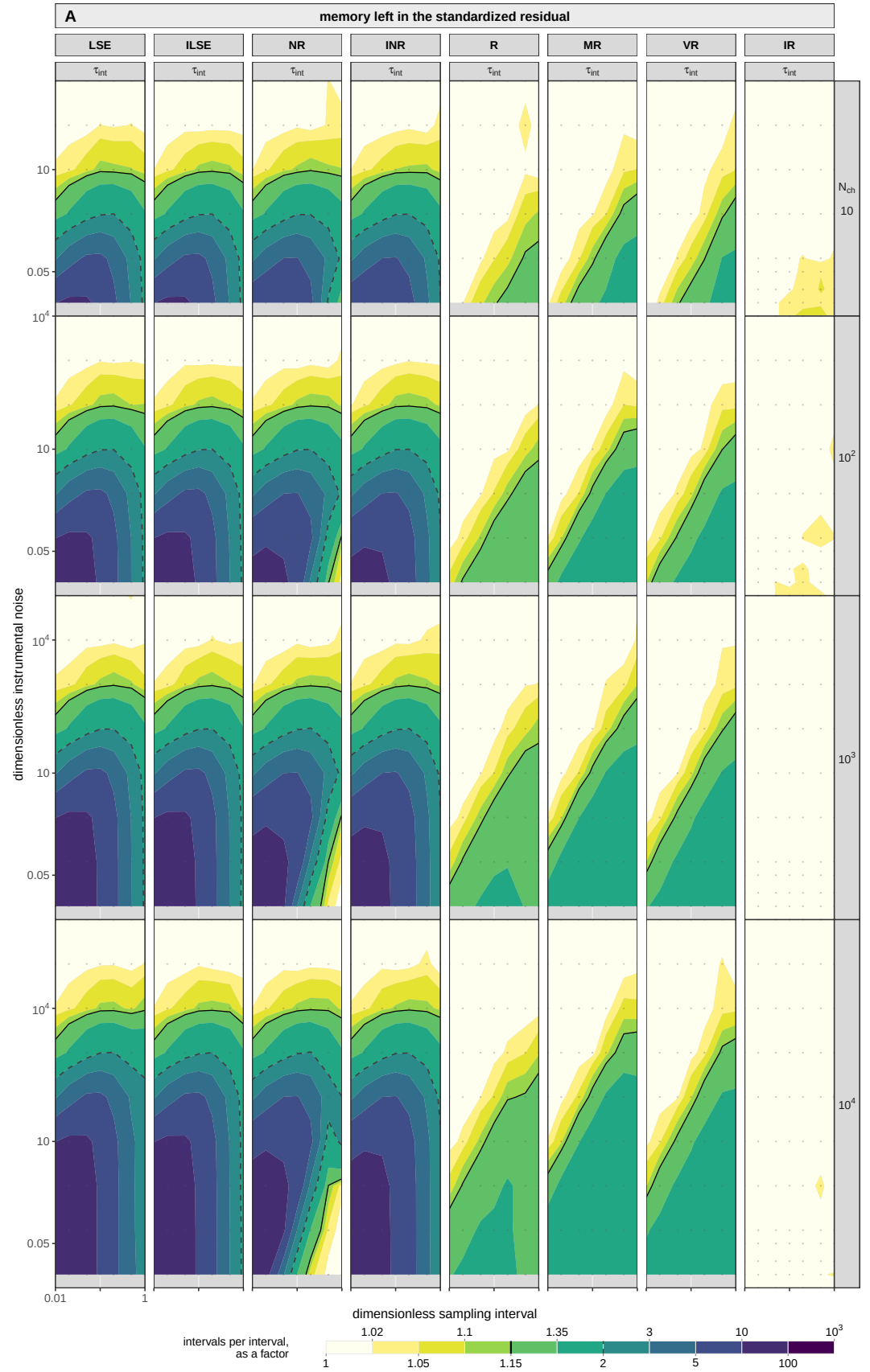
Figure 5—figure supplement 3. Where a recording leaves memory in its own residual. The horizontal axis of the figure above, drawn over the design plane instead of used as a coordinate: \tau_{int} , the integrated autocorrelation of the standardized residual in normalized form, for all eight members, one column each. It counts how many intervals a fit effectively has for every interval it believes it has, and reads one for a white residual. It is computed from the data against the member's own fitted mean and variance, with no parameter, no derivative and no comparison against another likelihood, which is what makes it the one quantity here an experimentalist can
