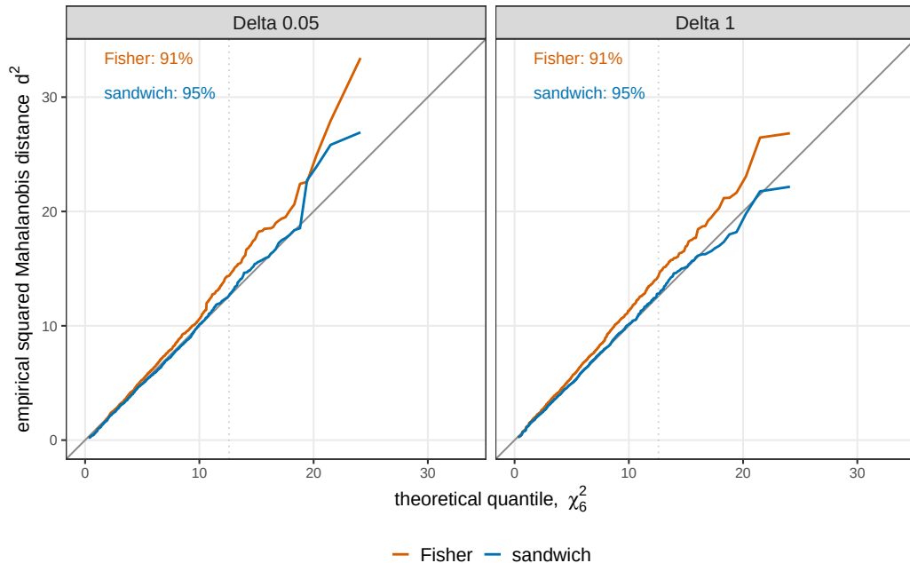
Sandwich vs reported covariance against the empirical MLE cloud (IR, N_ch 10, noise 0.05, 1000 fits, p = 6)
