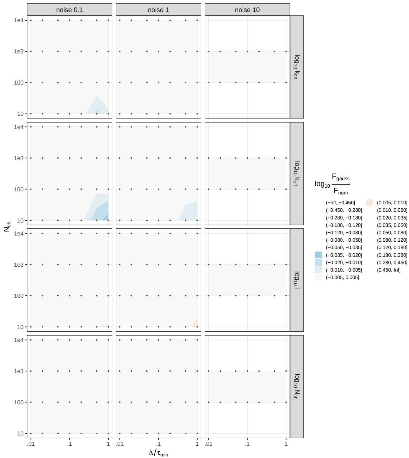
MNR Gaussian / numeric Fisher (diagonal), log10 ratio [pool]
