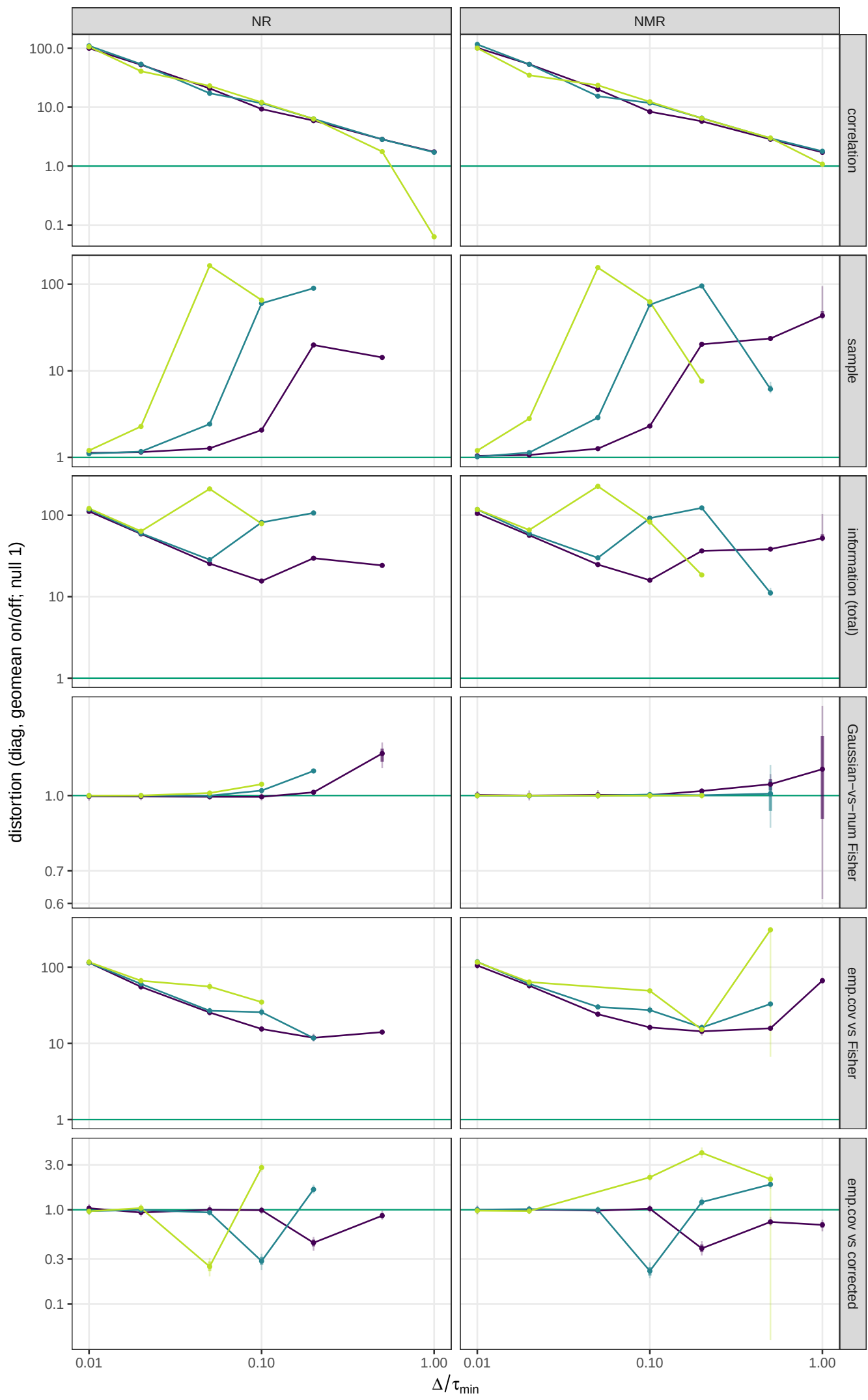
Figure 4-supplement Non-recursive NR, NMR (own scale)
