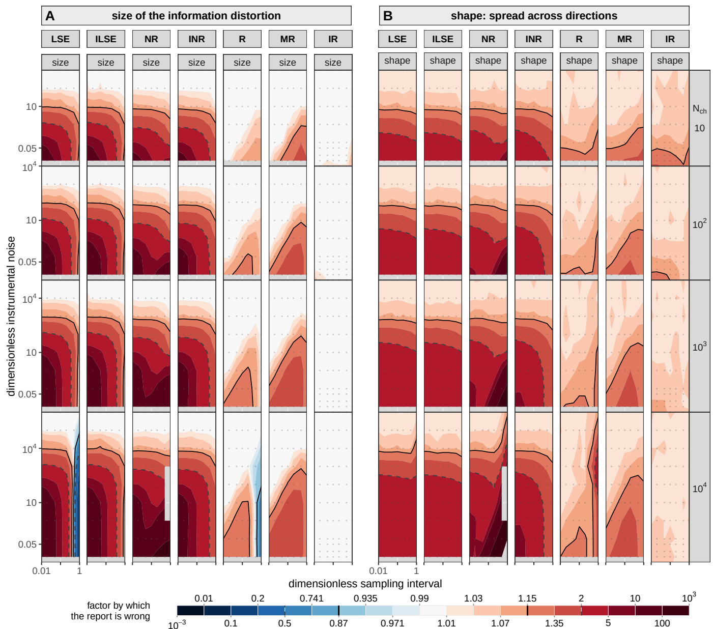
Figure 11. The magnitude of the information distortion against its anisotropy. Two invariants of the same distortion matrix over the same plane, for seven members: both least-squares arms, NR, INR, R, MR and IR. (A) its magnitude m and (B) its anisotropy a (Eq. 4), m signed about a null of one and a one-sided. The rule they give: a at one means a single effective-count rescaling is exact and m is the factor it should use; a above one means no such rescaling exists at any factor. The two least-squares arms are the same figure wherever the recording is finely sampled, and part at the coarsest interval: at \tilde{\Delta} = 1 and 10^4 channels LSE reads 0.074 in magnitude, understating its own information thirteenfold, where ILSE reads 1.00. That is the mean model failing and not the variance model, and it is the deepest of the few cells anywhere on this page where a member is conservative rather than overconfident: 11 of LSE's 210 cells and 4 of R's, all of them at the two coarsest intervals and none for any other member.
