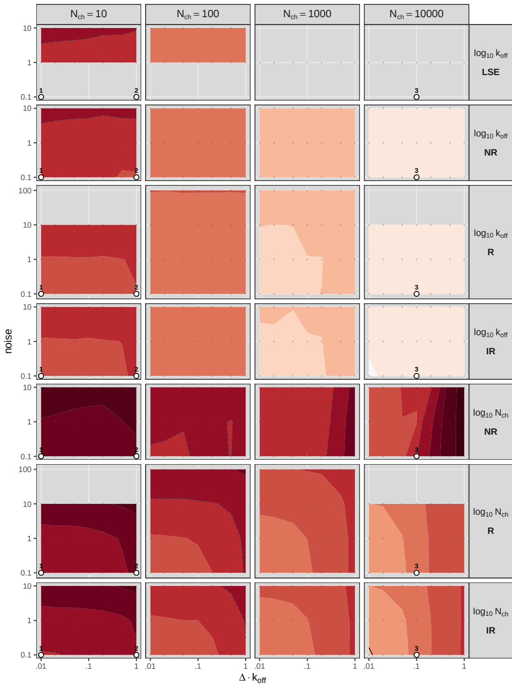
Distortion-corrected standard error
