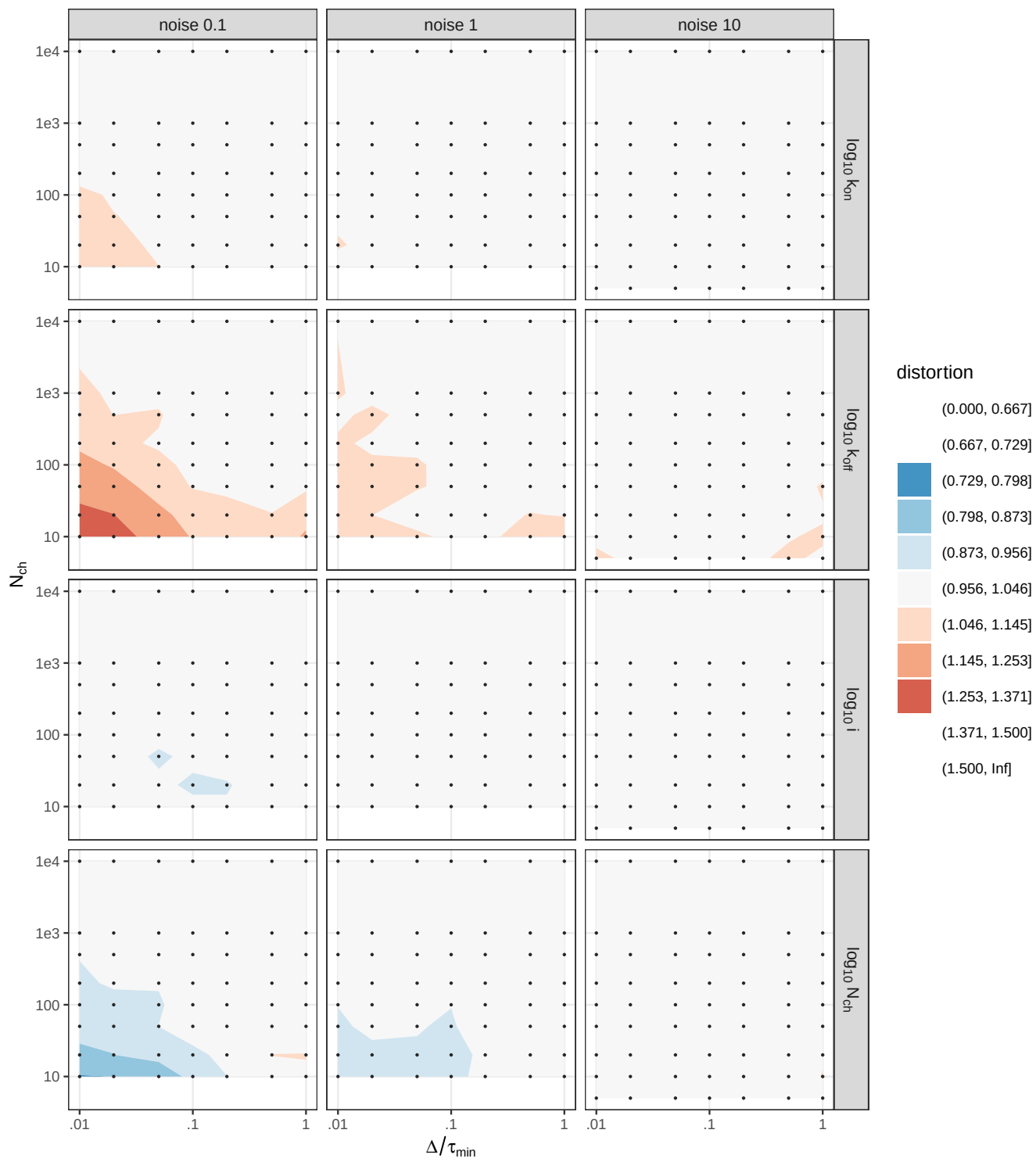
macro_IR Correlation distortion (diagonal) (filled)
