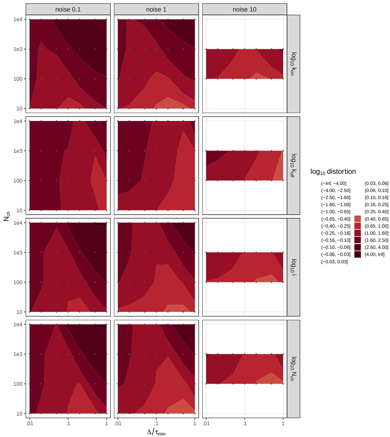
MNR Information distortion (diagonal), log 10 scale [sim]
