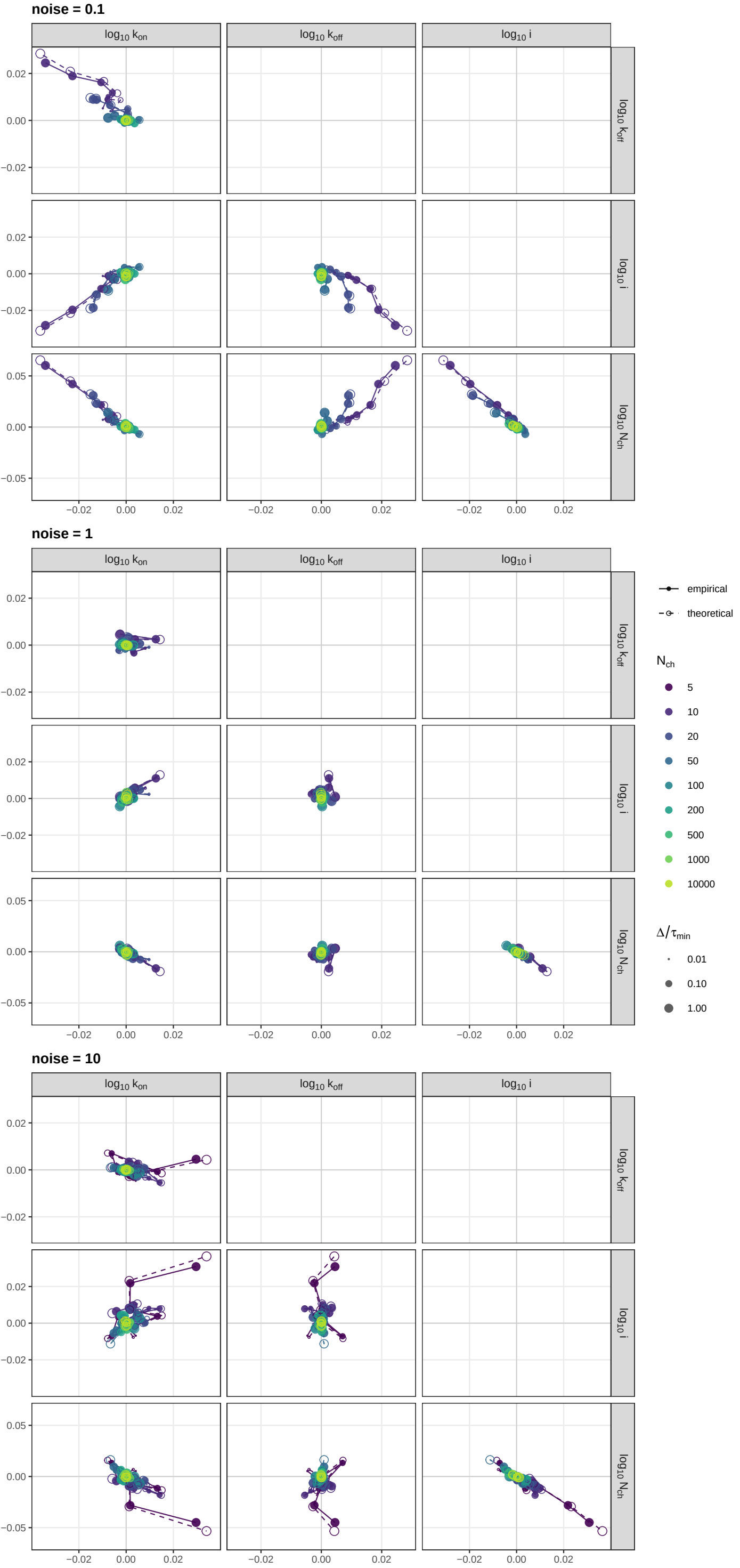
macro_IR parameter bias: empirical (solid, filled) vs theoretical DIB (dashed, open) log 10 units; colour = N ch , point size = interval
