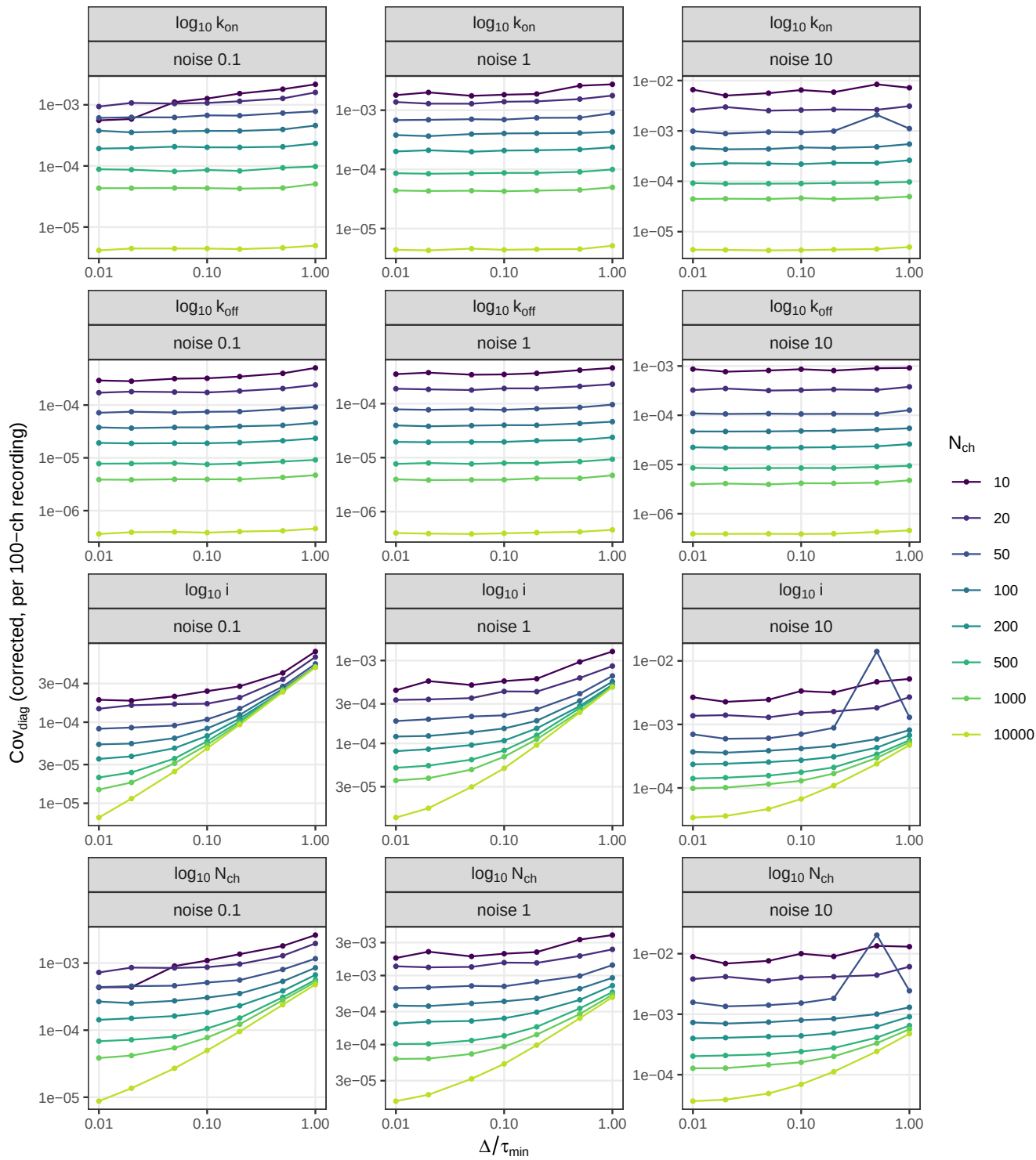
macro_IR corrected covariance (diagonal) vs interval, by N_ch
