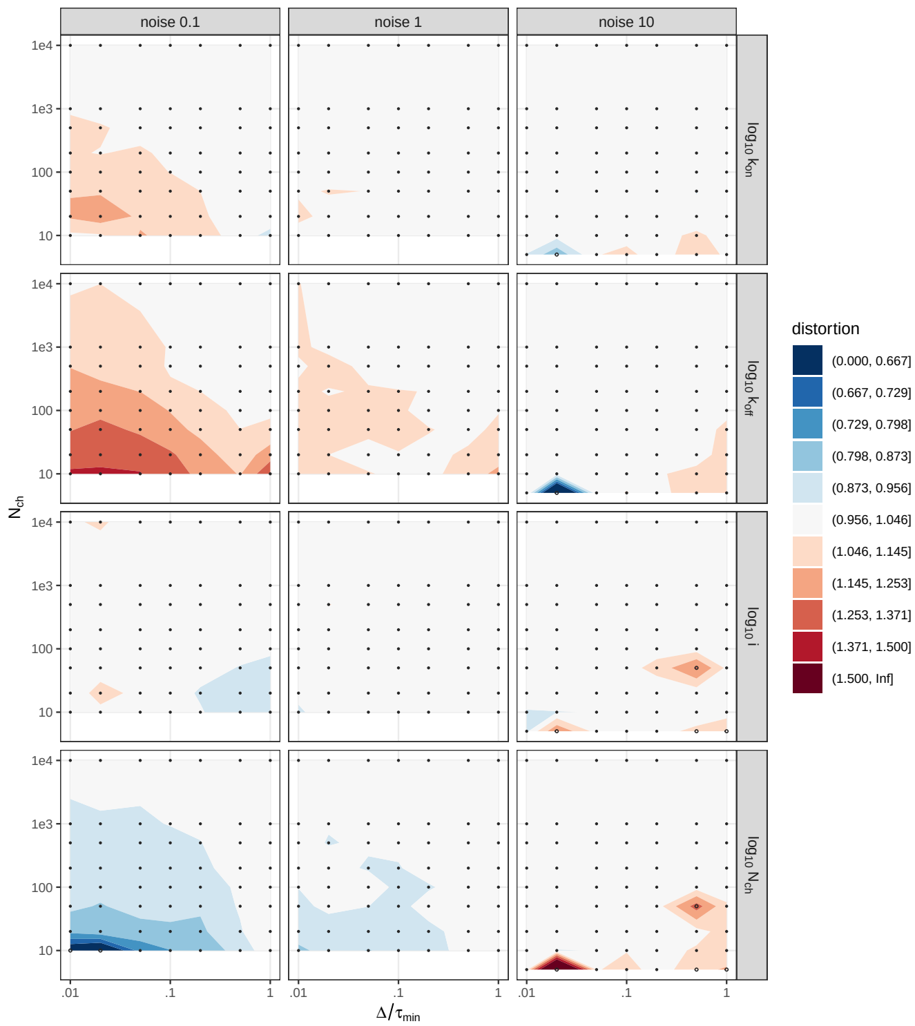
macro_IR Information distortion (diagonal) (filled)
