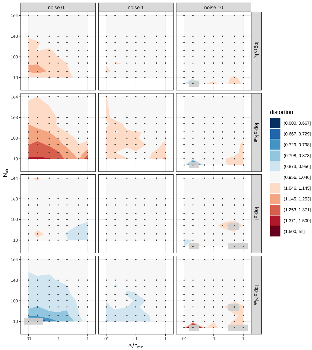
macro_IR Information distortion (diagonal) (grey = unreliable)
