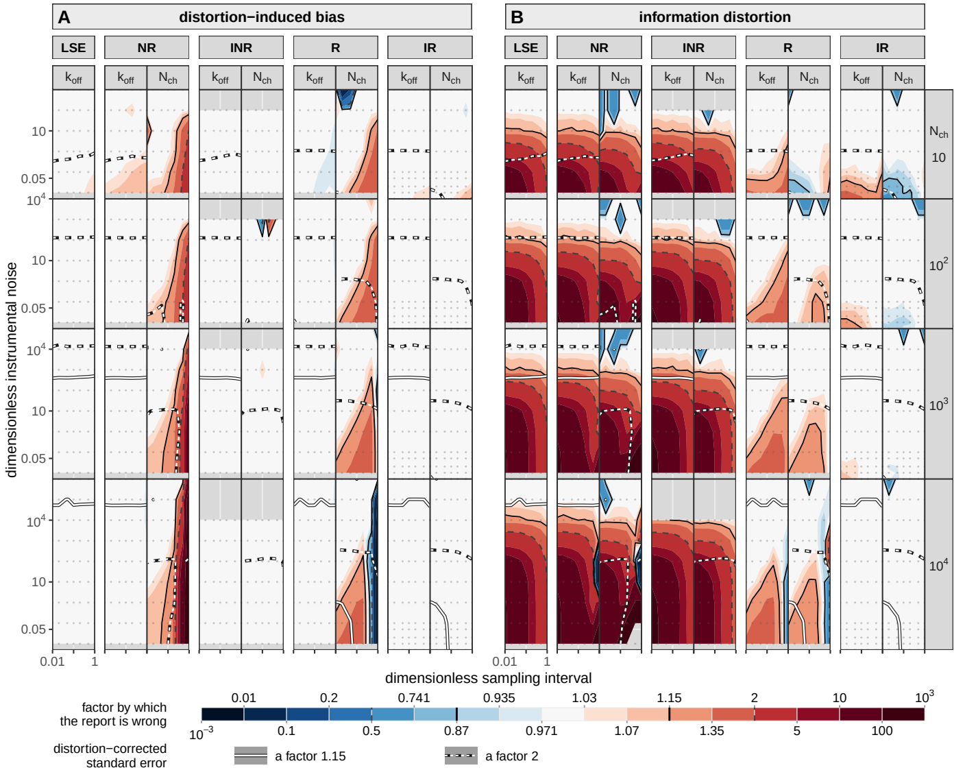
Figure 4. The design plane: how wrong each member's report is, in both moments, on one scale. Ten thousand recordings are simulated at every cell of the grid and scored by each member of the cost ladder. (A) The distortion-induced bias, evaluated at the simulation truth \theta_{\text{sim}} : how far the estimate is displaced. (B) The information distortion, evaluated at the pooled optimum \theta_{\text{pool}} , where the score vanishes by construction so a displaced gradient cannot contaminate it: how far the uncertainty a member reports is from the one it delivers. Columns nest twice, member and then parameter, k_{\text{off}} and N_{\text{ch}} . Least squares holds one column per half, because its four-parameter configuration fixes the unitary current and the noise level at the simulated values (Methods), so a channel-number comparison against it would not be like for like. Rows are the channel count, each given a height proportional to the range of instrumental noise the sweep reaches there, so a decade of noise is the same distance in every row. Inside a panel the axes are the sampling interval in units of \tau and the dimensionless instrumental noise, and one decade is the same physical distance on both, so a field's shape can be read as a shape. Colour is shared by the two halves: the factor by which the report is wrong, centred on one, pale right and saturated wrong in either direction, blue conservative. What a factor means differs between them and the difference is not cosmetic: in (A) it is a factor on the parameter, so 2 means the estimate is out by a factor of two, while in (B) it is a ratio of variances, so 2 means the reported error bar is \sqrt{2} , about 40%, too narrow. The scale is clipped at 10^{\pm 3} , which touches 22 of 3276 cells, twenty of them the open-loop member, where being wrong by 10^3 and by 10^{12} say the same thing. Lines carry two codes: colour says which quantity, dark hairlines cutting the colour field and white lines on a dark casing cutting the distortion-corrected standard error, which asks whether the parameter can be measured at all rather than whether its error bar is honest; dash says which criterion, solid a factor 1.15 and dashed a factor 2, the two thresholds used throughout. Both criteria are edges of the colour bands, which is why the dark pair needs no key of its own.
