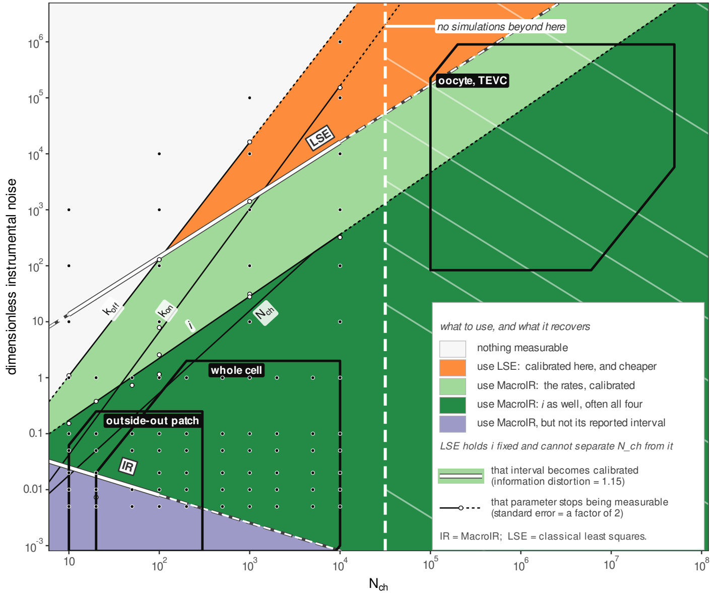
Figure 6. What a macroscopic recording can be asked for: a usage map over channel number and instrumental noise. The plane is the design space, the number of channels in the patch against the instrumental noise label, both on logarithmic scales, at one acquisition interval \Delta \cdot k_{off} = 0.1 . Four boundaries divide it, and they are two questions asked of two methods. Colour is the parameter the boundary is about. Line type is the question: solid asks whether the parameter can be measured at all, drawn where the distortion-corrected standard error crosses a factor of two; dotted asks whether the reported error bar of least squares is honest, drawn where its information distortion crosses 1.15; dashed asks the same of the likelihood's own error bar, and is the boundary below which the Gaussian closure is misspecified. Ribbons are the same boundary swept over acquisition intervals from 0.01 to 1 in units of \tau , so a ribbon says where a reader's own sampling rate puts the boundary and is not an error bar. Dots are the measured crossings and the line through them is their fitted power law, drawn faint where it leaves the simulated range, which is marked. Vertical strips mark the two vertices, each a range set by the strict and the loose criterion. The boundaries partition the plane into five regions, filled and keyed by what a recording in each can be asked for, and the three labelled boxes mark where common preparations sit; the regions are named and read in order in the text. The map is a concept map, not a phase diagram. Its boundaries are level sets of continuous diagnostics, so a looser criterion moves each of them by up to a decade in noise without changing the layout.
