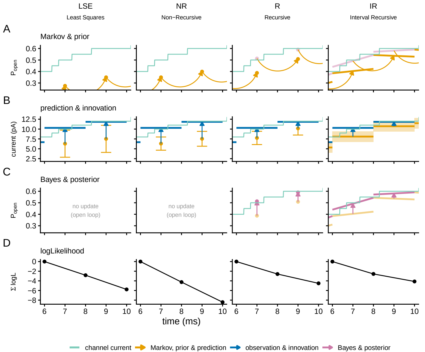
Figure 1. One filter step along the cost ladder. The current from a patch of N_{\text{ch}} = 20 two-state channels, recorded as an interval average with white instrumental noise, is scored by each of the four body members (columns): least squares on the deterministic mean current (LSE), the open-loop gating likelihood (NR), the recursive filter on instantaneous samples (R), and the boundary-conditioned filter (IR). Rows follow one turn of the cycle: (A) the prior open probability from the Markov step, (B) the predicted current with its spread and the innovation, (C) the Bayesian posterior, which for the two non-recursive columns reads as no update, and (D) the per-step log-likelihood accumulated over the window and reset at the window start. Two measurement windows are shown (6 to 10 ms of a 12 ms recording). LSE is drawn in NR's grammar, a point mean with an error bar, so that its constant least-squares variance can be read against NR's per-interval gating variance. Colour encodes the filter phase and is shared across rows: green the simulated channel current, orange the predict phase, blue the observation and the innovation, purple the update, black the log-likelihood. A quantity carried in from the neighbouring interval is drawn hollow or dashed. Three of the seven rungs are not drawn, because the form of the cycle does not change for them; the one step that does change form, the gain acquiring the boundary term, is the R-to-IR step drawn here. Appendix 1 writes all seven out and says why the other three add no new step. The recording is one 20-channel trace simulated with 250 within-interval substeps and does not enter any quantitative comparison.
