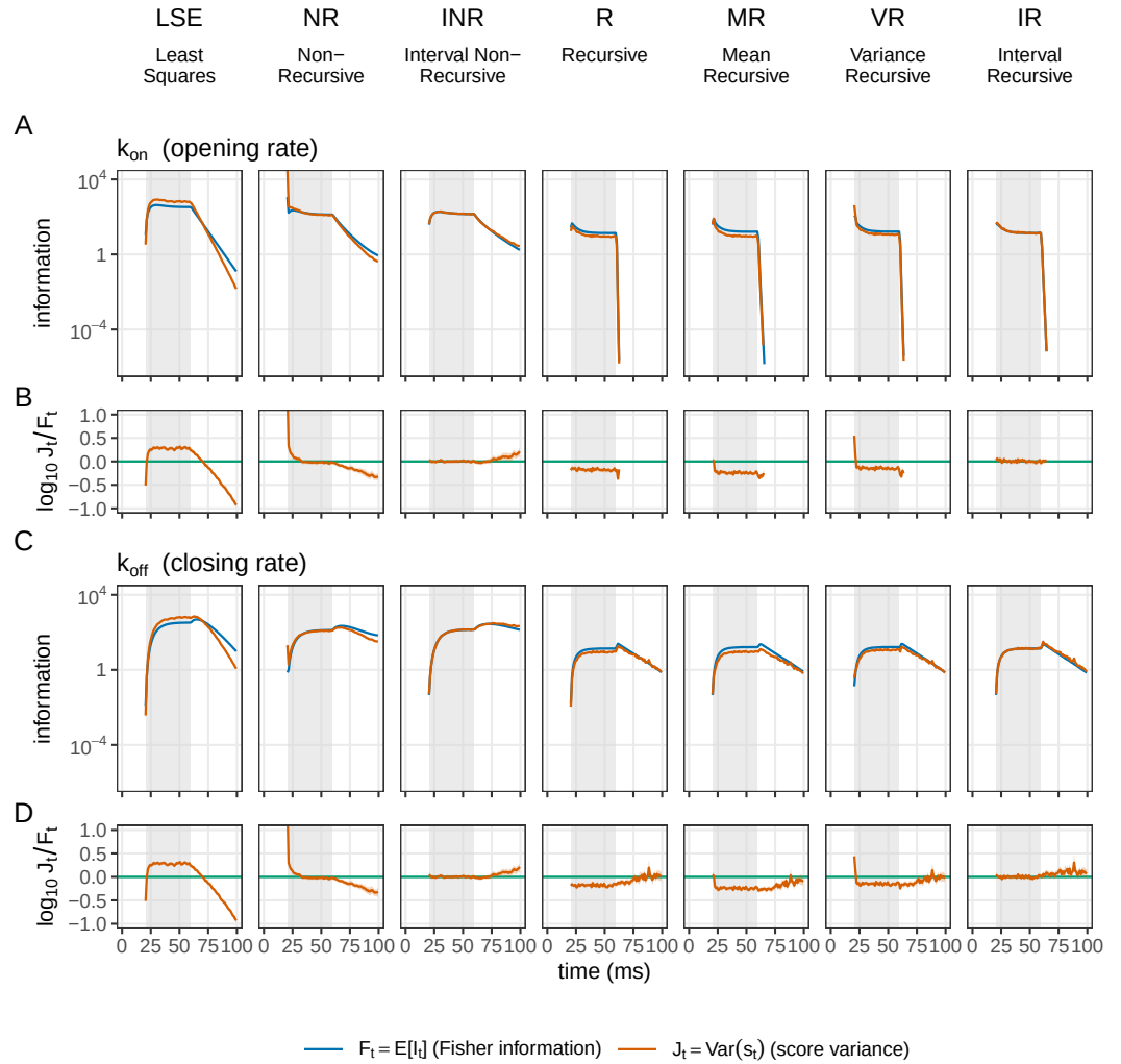
Figure 3—figure supplement 1. Per-step information against score variance, the opening rate and the closing rate. All seven members across the columns and two parameters down the page as bands of two rows: k_{on} (A, B) and k_{off} (C, D). The upper row of each band carries the per-interval Fisher information and the score variance as magnitudes, which lie on each other where the member is calibrated at that interval; the lower row is \log_{10}(J_t/F_t) with its 95% bootstrap interval, zero when they do. Per-interval calibration is not monotone along the cost ladder: on k_{off} the median reads +0.184 for LSE, -0.038 for NR, +0.007 for INR, -0.145 for R, -0.229 for MR, -0.135 for VR and +0.033 for IR, so the cheapest member that models the interval average is better calibrated interval by interval than any of the three recursive members that cost more. Curves stop at the information mask, which is also where the upper axis ends. In the two recursive columns the k_{on} band reaches that floor within six intervals of the agonist being removed while the k_{off} band does not. The least-squares ratio row is the same curve in every band of both halves, with a median of 0.183889 in each: with a single constant variance the parameter cancels out of the ratio, which leaves the true residual variance over the assumed one.
