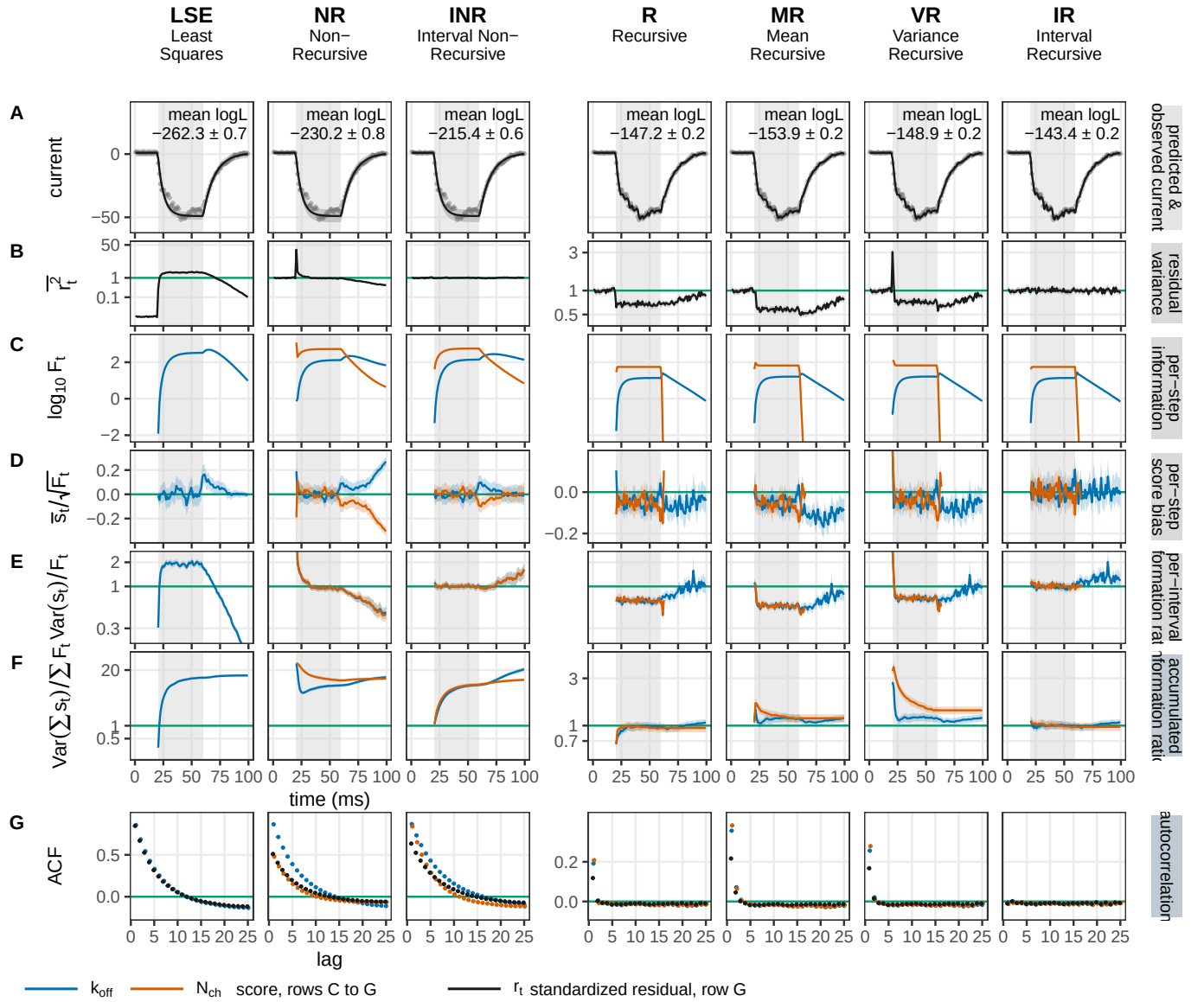
Figure 3. The calibration cascade in time, over the whole implemented family. One set of 1,000 recordings ( N_{\text{ch}} = 100 , noise label 0.1, \Delta \cdot k_{\text{off}} = 0.1 ) is scored by each of the seven members (columns, in cost-ladder order), with no fitting. Rows A and B are properties of the data, in grey; rows C to G are per parameter, the closing rate and the channel number in colour. (A) An example recording with the predicted current, its band the filter's own predictive \pm 1 s.d., annotated with the ensemble-mean log-likelihood and its standard error. (B) The mean squared standardized residual, one when the predictive variance is right. (C) The per-interval Fisher information, so where each parameter is measured. (D) The mean per-interval score over \sqrt{F_t} , zero when unbiased and standardized so parameters with different units share an axis. (E) The per-interval information ratio \text{Var}(s_t)/F_t , one at each interval. (F) The same ratio accumulated, J_T/F_T . (G) The autocorrelation against lag of the standardized residual, in black, and of the score for each parameter, in its colour; the score's is why (E) holds where (F) does not, and the residual's is the same memory in the data and the only quantity here an experimentalist can compute on a real recording. Bands are 95% bootstrap intervals over the recordings; curves stop where the information reaches zero. Non-negative quantities are on a logarithmic axis with the calibrated value on the ticks, signed quantities on a linear axis with zero on the ticks; the three open-loop columns share a y-scale block distinct from the four recursive ones. The channel number is not drawn for least squares, which cannot separate it from the unitary current.
