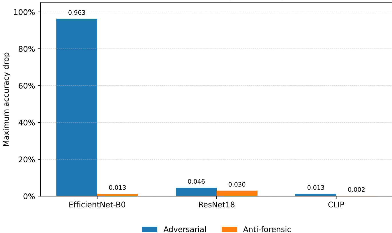
Maximum robustness degradation by model
