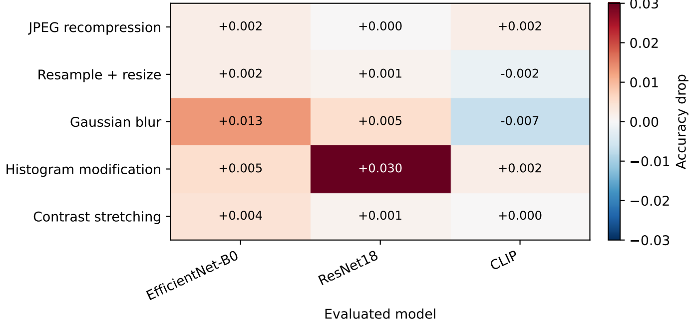
Accuracy drop under anti-forensic transformations
