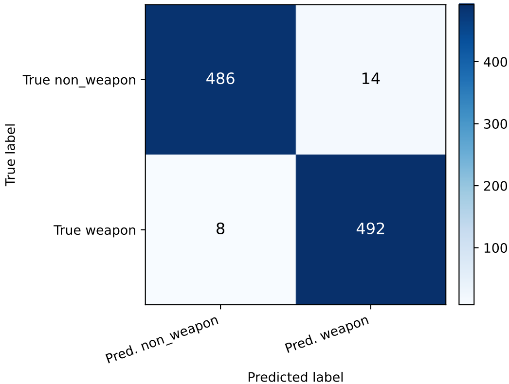
Clean confusion matrix — EfficientNet-B0
