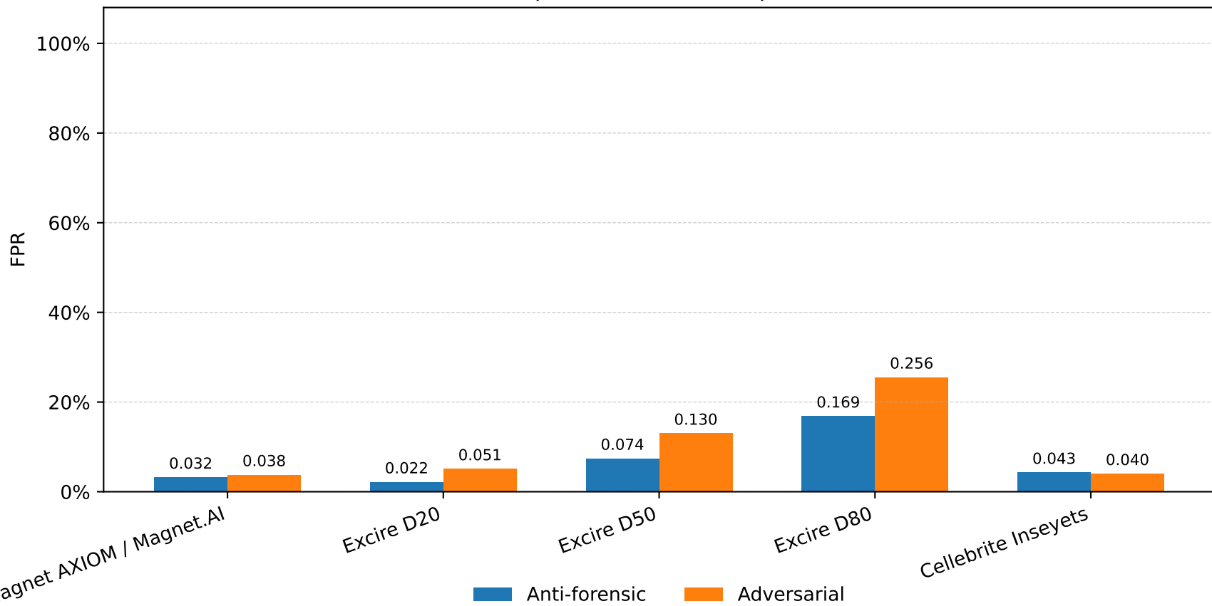
Forensic-tool false positive rate under perturbation families
