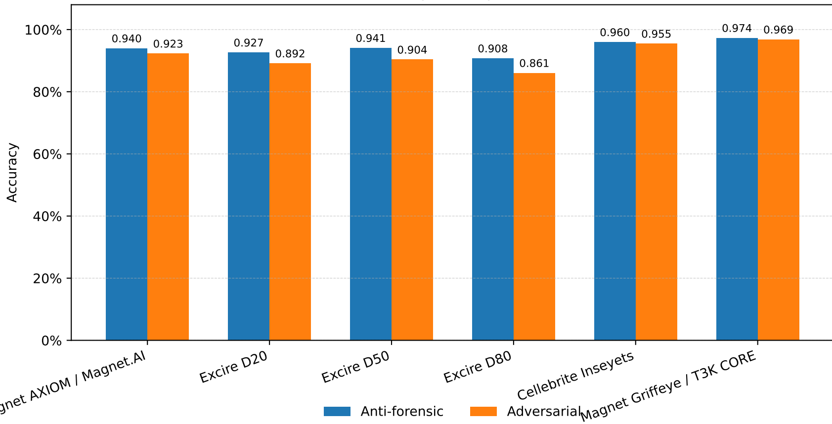
Forensic-tool accuracy under perturbation families
