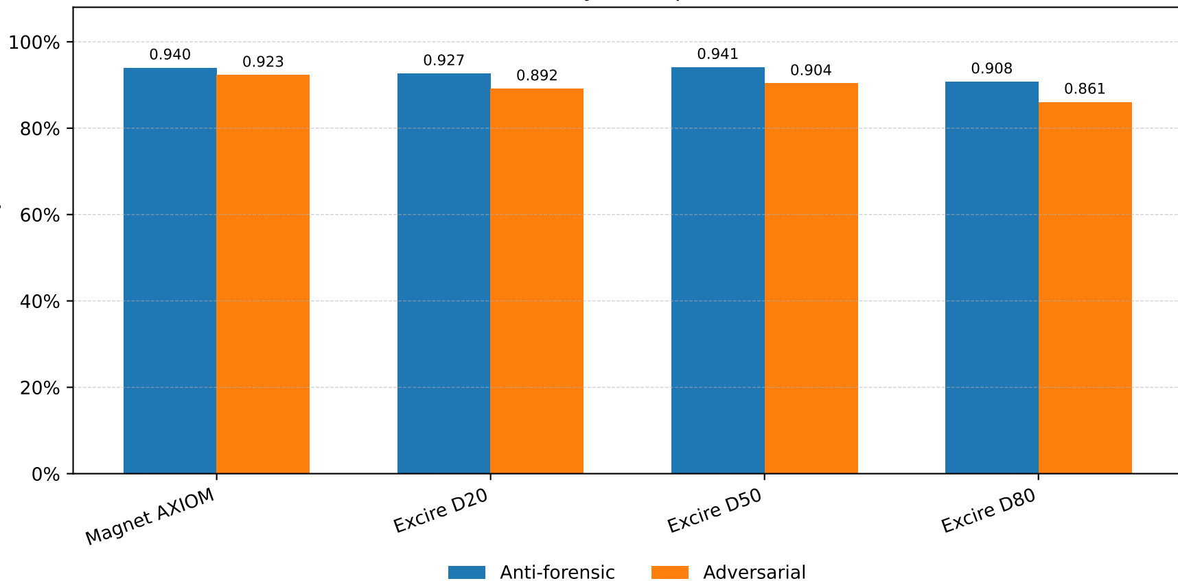
Forensic-tool accuracy under perturbation families
