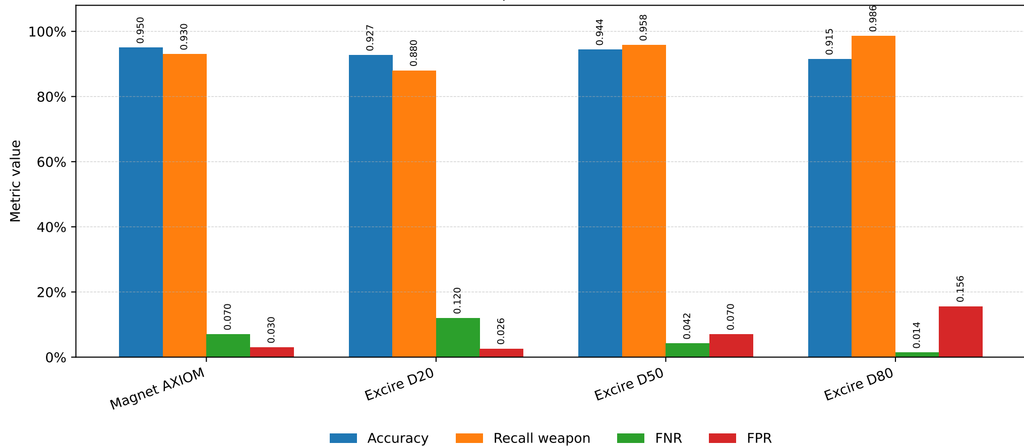
Clean-set comparison of forensic AI tools
