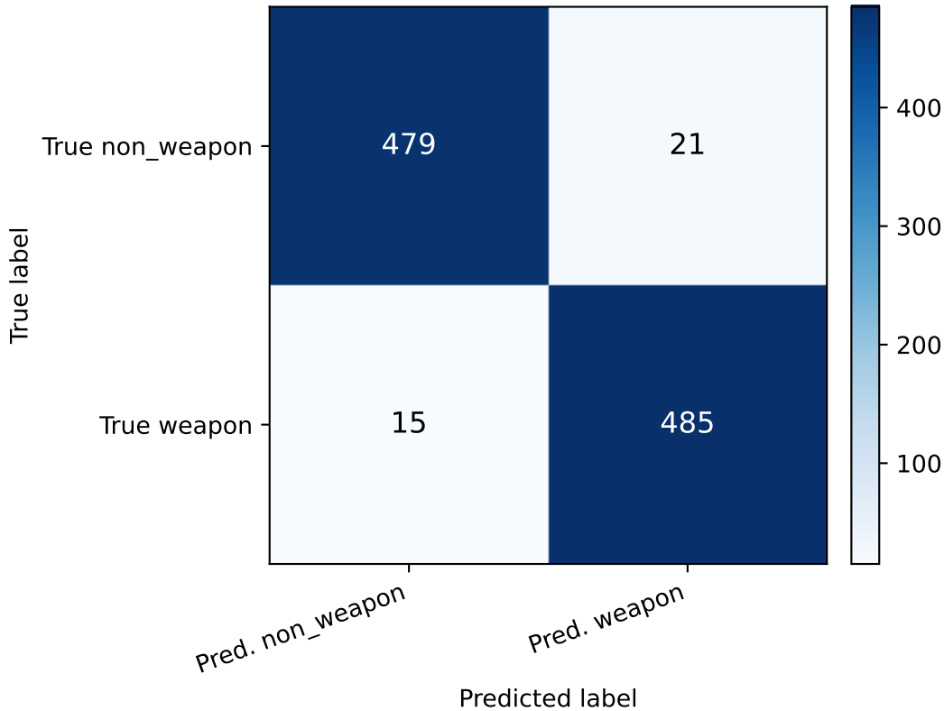
Clean confusion matrix — ResNet18
