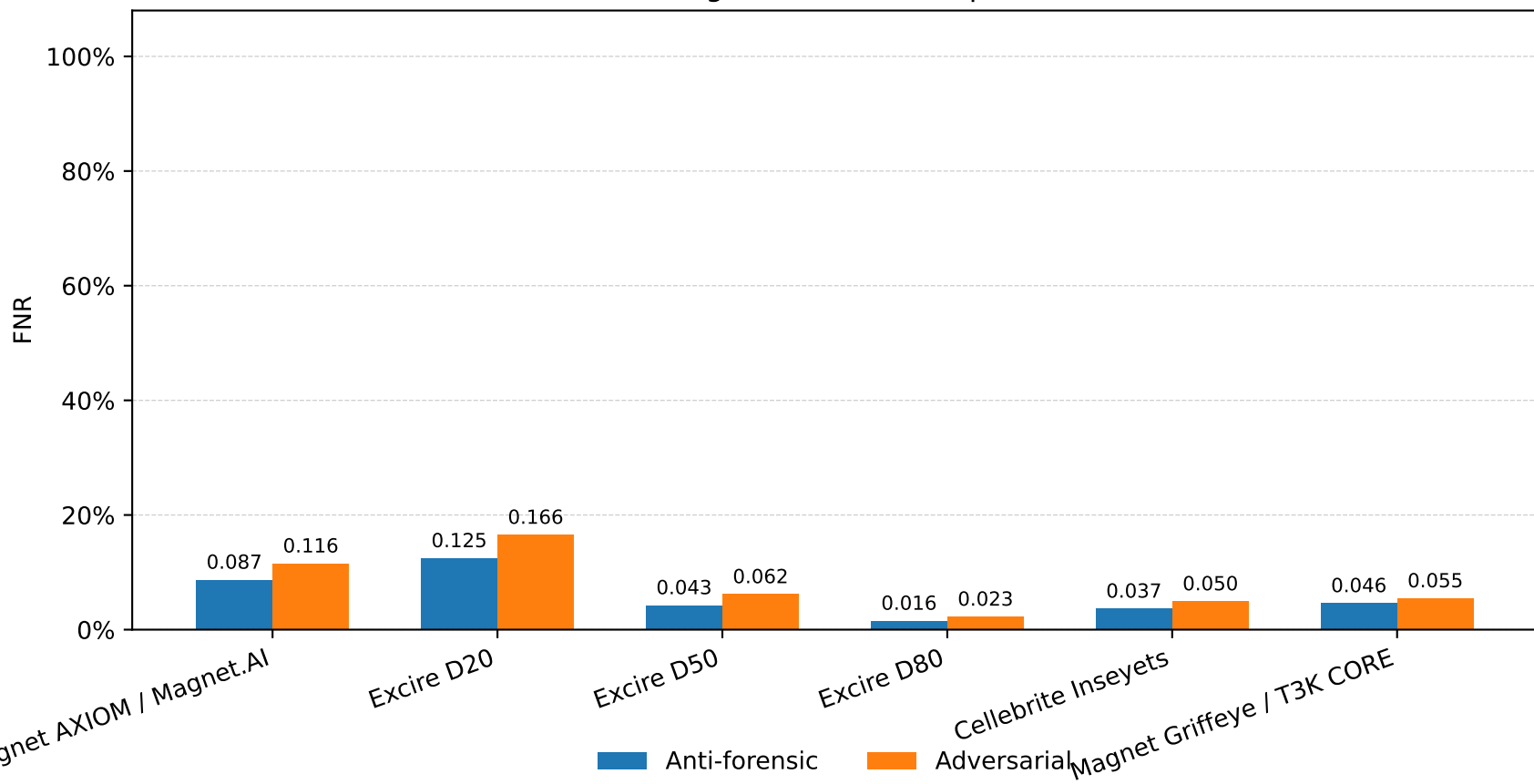
Forensic-tool false negative rate under perturbation families
