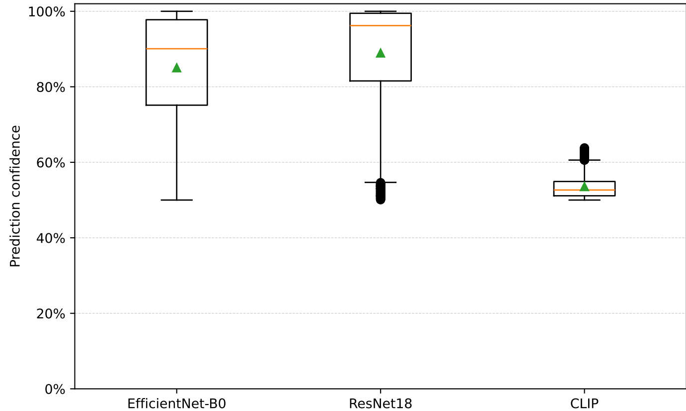
OOD confidence distribution by proxy model
