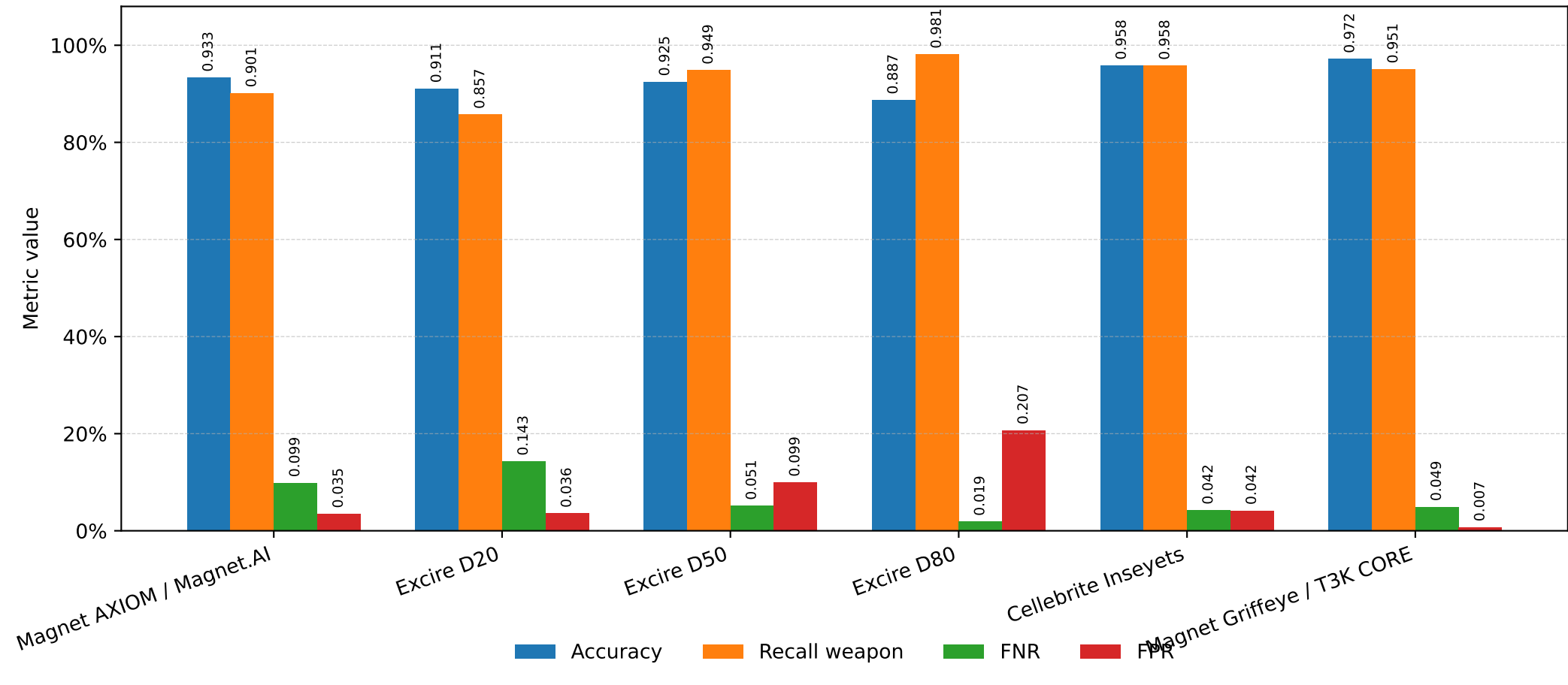
Overall comparison of black-box forensic AI tools
