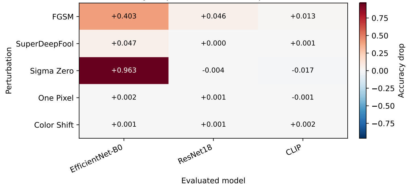
Accuracy drop under adversarial perturbations
