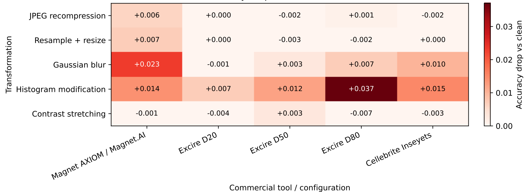
Forensic-tool accuracy drop under anti-forensic transformations
