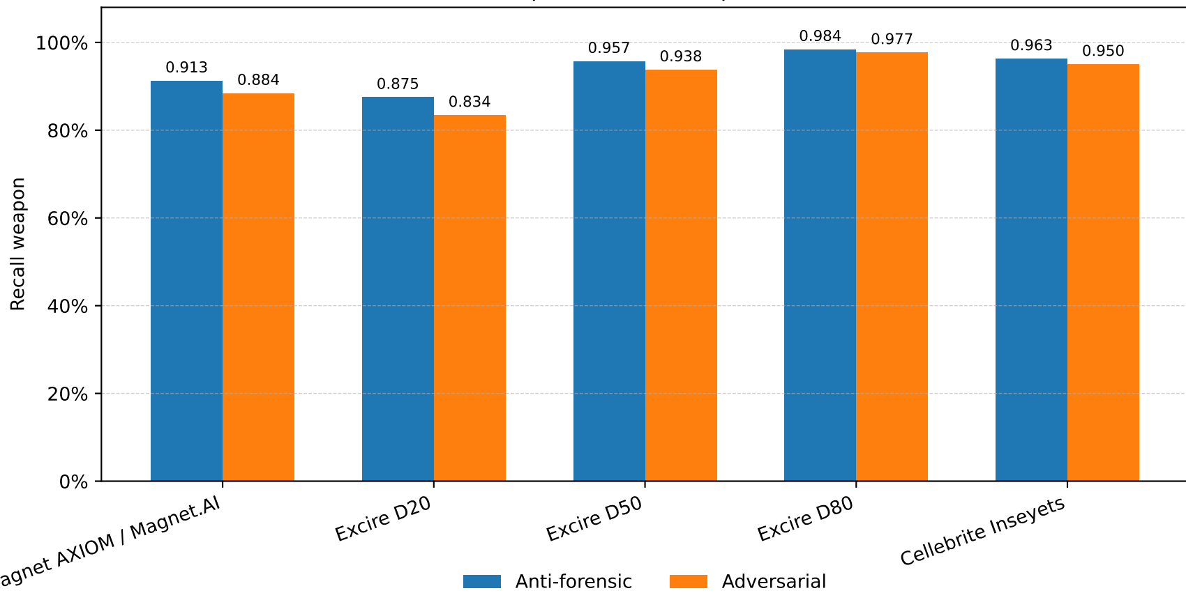
Forensic-tool weapon recall under perturbation families
