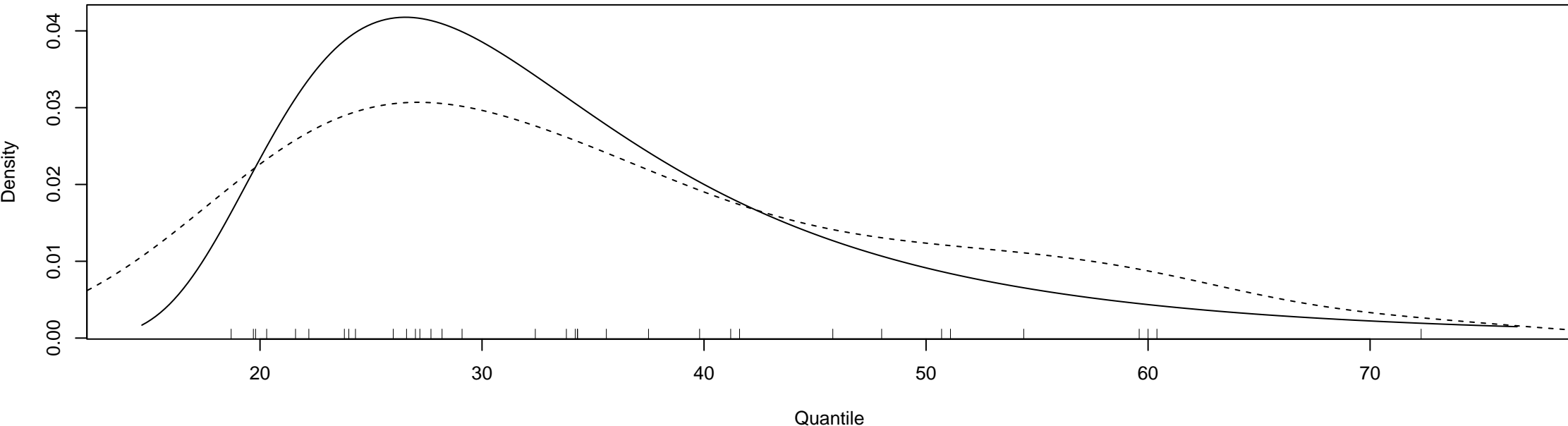
Density Plot
