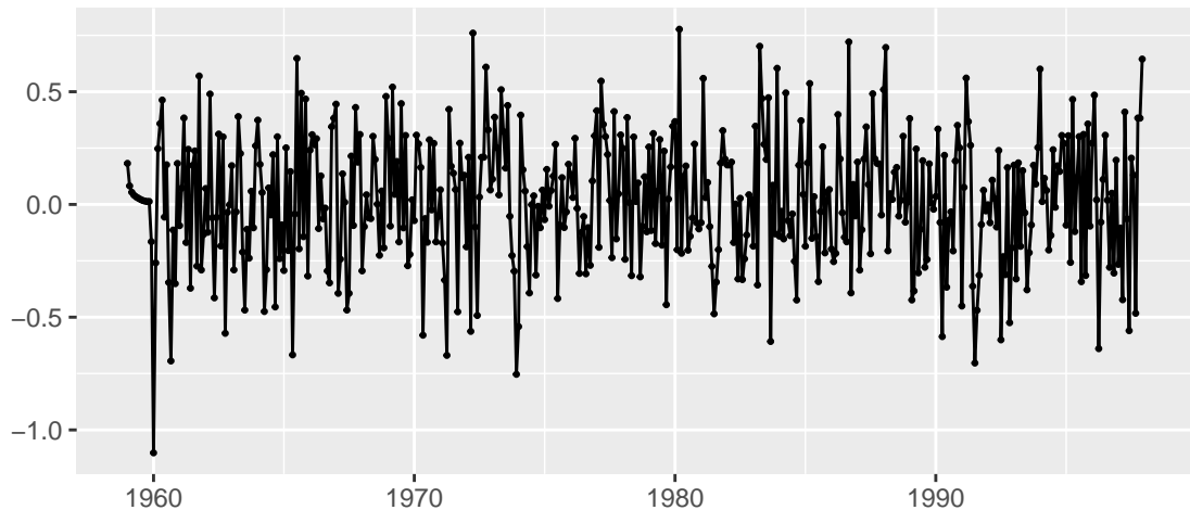
Residuals from ARIMA(1,1,1)(1,1,2)[12]
