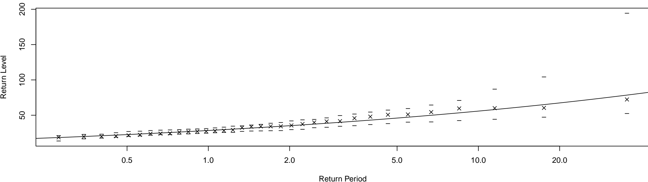
Return Level Plot
