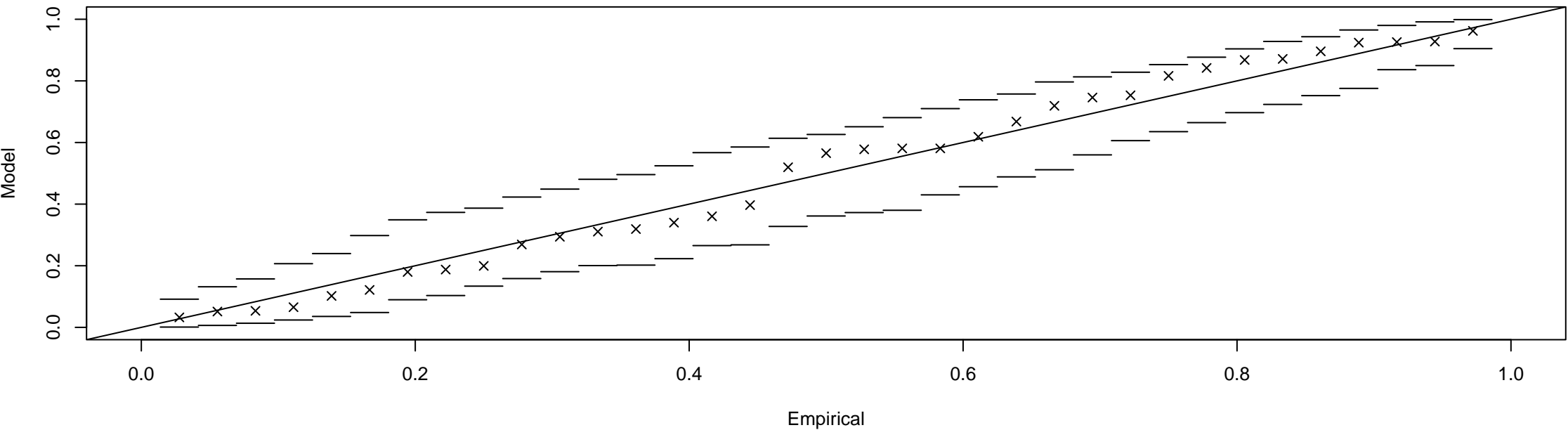
Probability Plot
