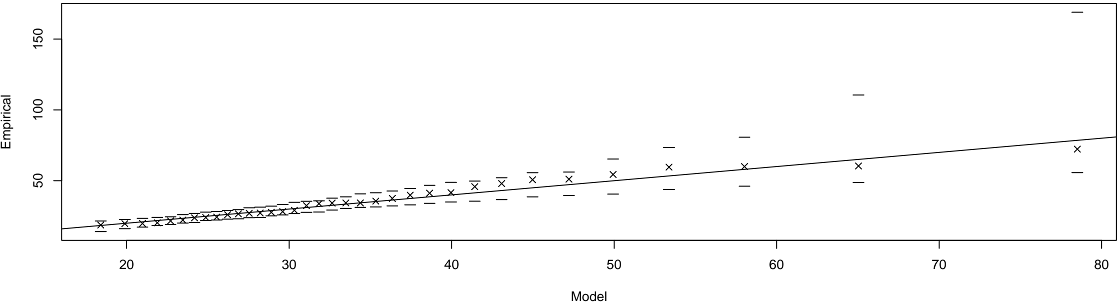
Quantile Plot
