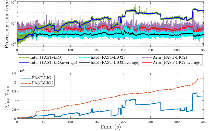
Fig. 8. Processing time for each LiDAR scan of FAST-LIO and FAST-LIO2.
