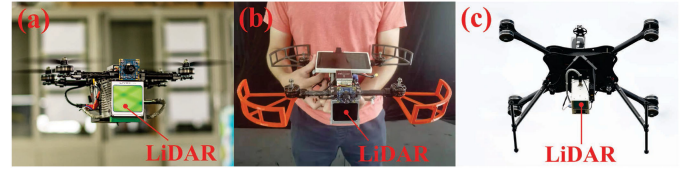
Fig. 6. Three different platforms. (a) Small-scale quadrotor UAV with 280-mm wheelbase carrying a forward-looking Livox Avia LiDAR. (b) Handheld platforms. (c) Quadrotor UAV 750-mm wheelbase carrying a down-facing Livox Avia LiDAR. All three platforms carry the same DJI Manifold-2 C onboard computer. The video of real-world experiments is available online (see footnote 8).
