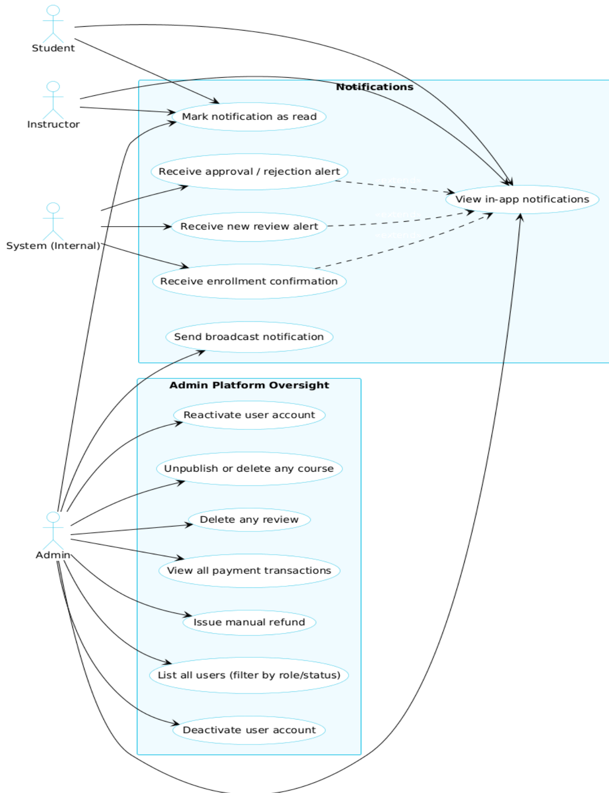
Figure 4 — Notifications & Admin Platform Oversight Use-Case Diagram
