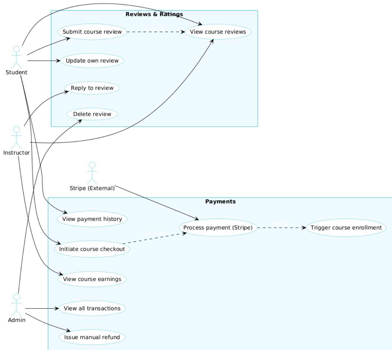
Figure 3 — Payments &amp; Reviews Use-Case Diagram
