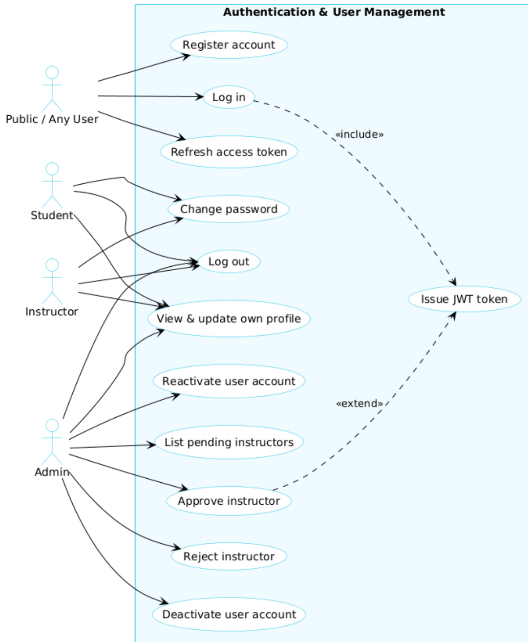
Figure 1 — Authentication & User Management Use-Case Diagram
