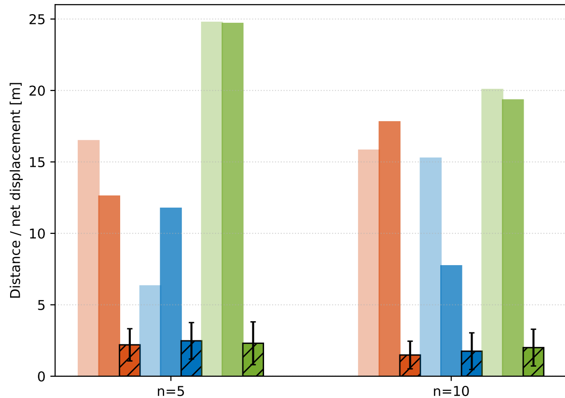
Distance: sim (10m arena, light) vs sim (3.5m arena, solid) vs hardware net displacement (hatched)
