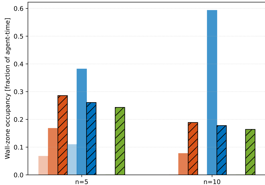
Wall proximity: sim (10m, light) vs sim (3.5m, solid) vs hardware brake-zone (hatched)
