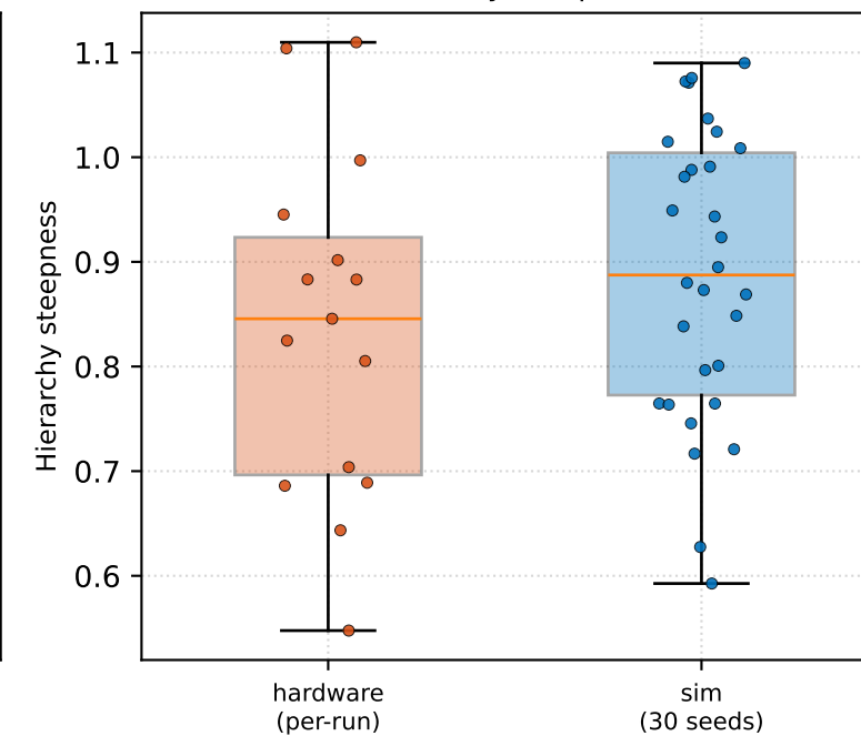
Metric 2 -- directional-correlation hierarchy steepness
