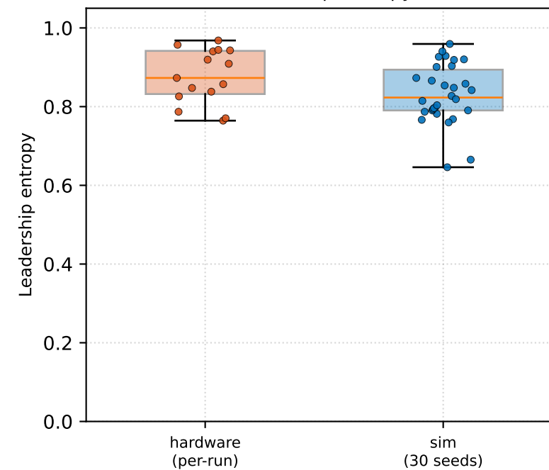
Metric 2 -- directional-correlation leadership entropy
