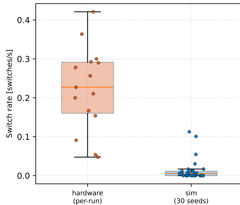
Metric 4 -- persistence-filtered hand-off rate
