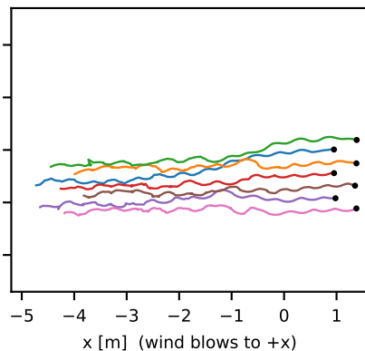
Baseline (rep5)
