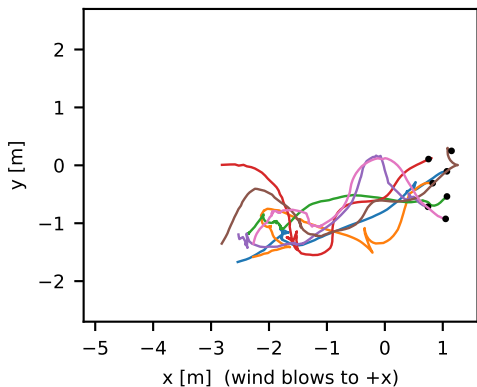
Stage 2 (rep28)
