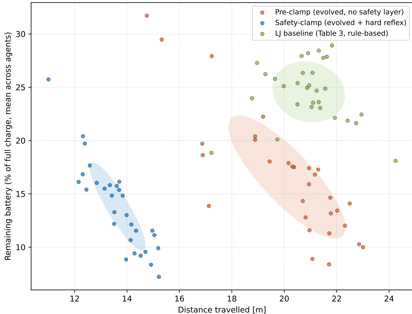
Fig. 5a analog -- distance vs. remaining battery (30 runs/condition, n=10)
